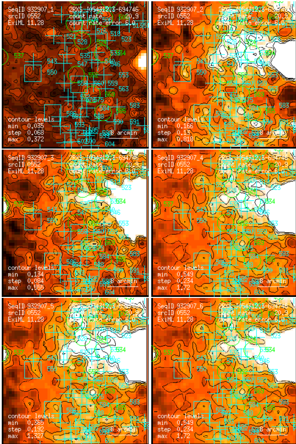
Figure 552: RASS 932907: detection 0552: band rate images, Gaussian filter: (1) PSPC channels 11 – 41, (2) 52 – 90, (3) 91 – 201, (4) 11 – 235, (5) 52 – 201, (6) 11 – 201. Broad band rates in counts/ks. Band rate contour levels in counts/ks/arcmin 2 .
