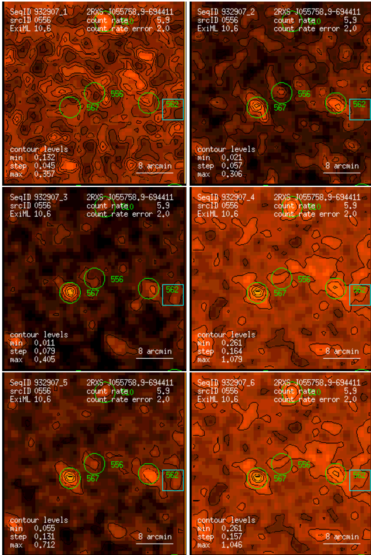
Figure 556: RASS 932907: detection 0556: band rate images, Gaussian filter: (1) PSPC channels 11 – 41, (2) 52 – 90, (3) 91 – 201, (4) 11 – 235, (5) 52 – 201, (6) 11 – 201. Broad band rates in counts/ks. Band rate contour levels in counts/ks/arcmin 2 .
