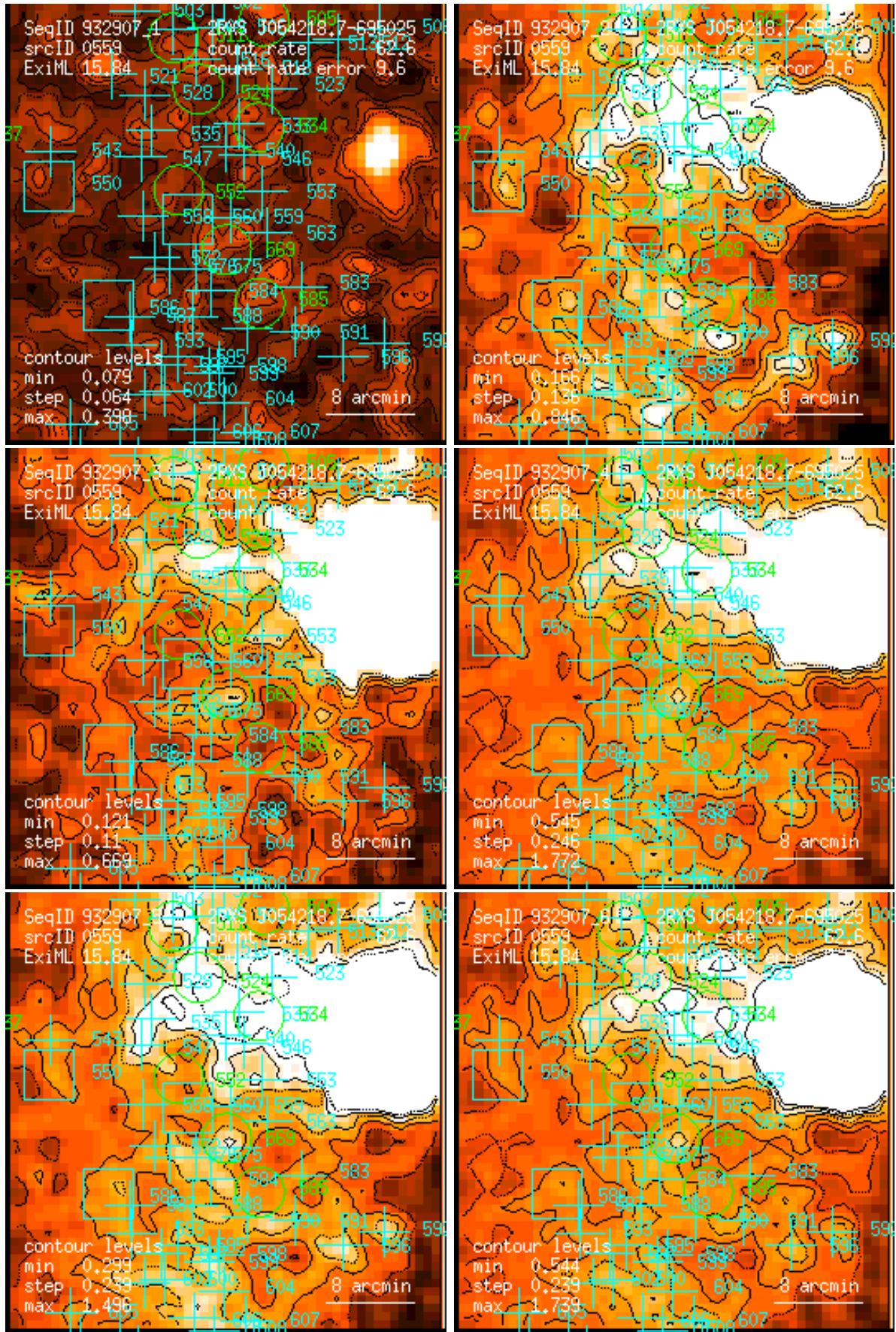
Figure 559: RASS 932907: detection 0559: band rate images, Gaussian filter: (1) PSPC channels 11 – 41, (2) 52 – 90, (3) 91 – 201, (4) 11 – 235, (5) 52 – 201, (6) 11 – 201. Broad band rates in counts/ks. Band rate contour levels in counts/ks/arcmin 2 .
