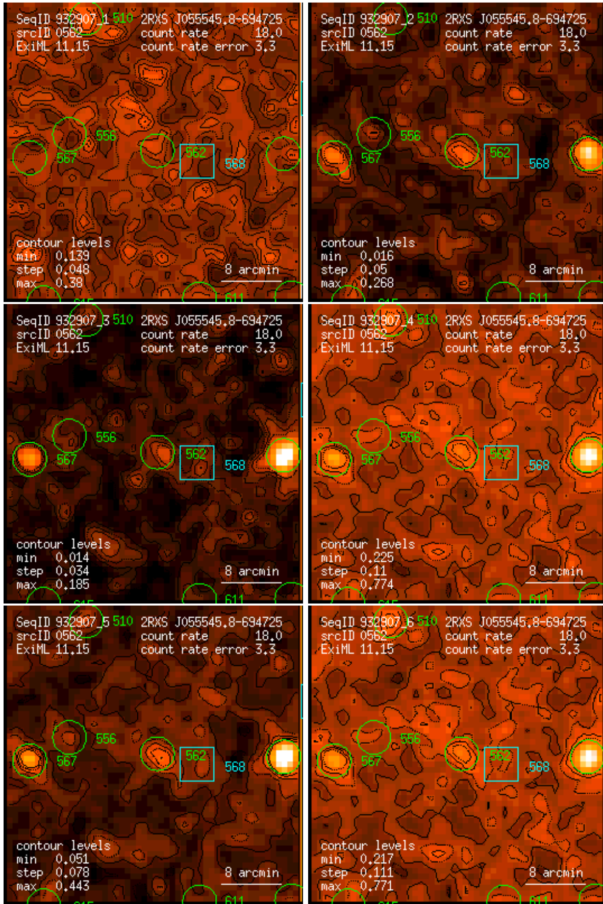
Figure 562: RASS 932907: detection 0562: band rate images, Gaussian filter: (1) PSPC channels 11 – 41, (2) 52 – 90, (3) 91 – 201, (4) 11 – 235, (5) 52 – 201, (6) 11 – 201. Broad band rates in counts/ks. Band rate contour levels in counts/ks/arcmin 2 .
