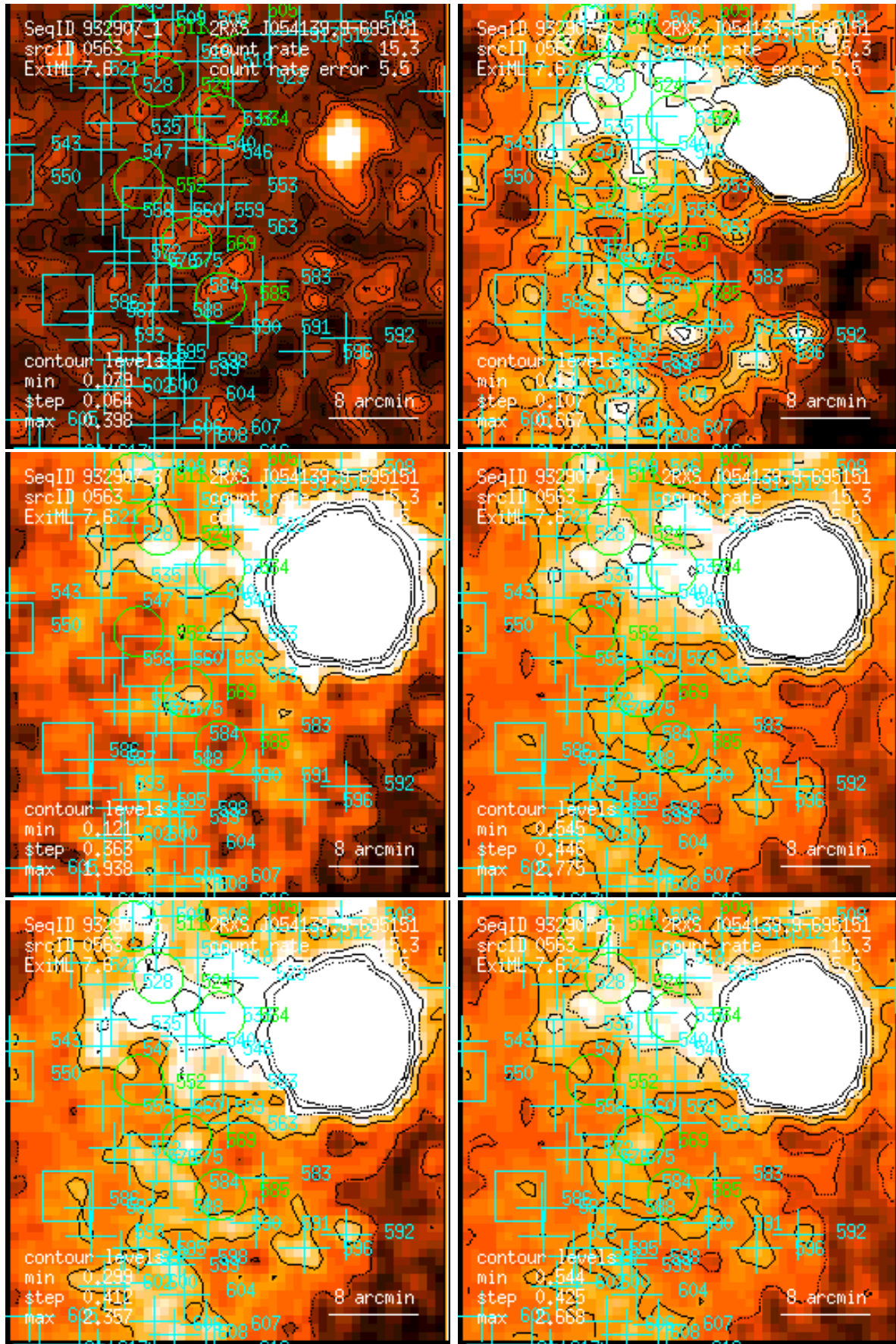
Figure 563: RASS 932907: detection 0563: band rate images, Gaussian filter: (1) PSPC channels 11 – 41, (2) 52 – 90, (3) 91 – 201, (4) 11 – 235, (5) 52 – 201, (6) 11 – 201. Broad band rates in counts/ks. Band rate contour levels in counts/ks/arcmin 2 .
