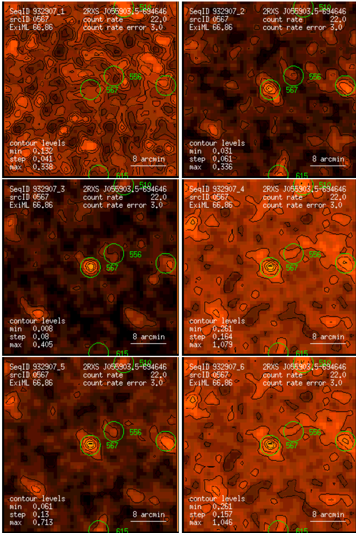
Figure 567: RASS 932907: detection 0567: band rate images, Gaussian filter: (1) PSPC channels 11 – 41, (2) 52 – 90, (3) 91 – 201, (4) 11 – 235, (5) 52 – 201, (6) 11 – 201. Broad band rates in counts/ks. Band rate contour levels in counts/ks/arcmin 2 .
