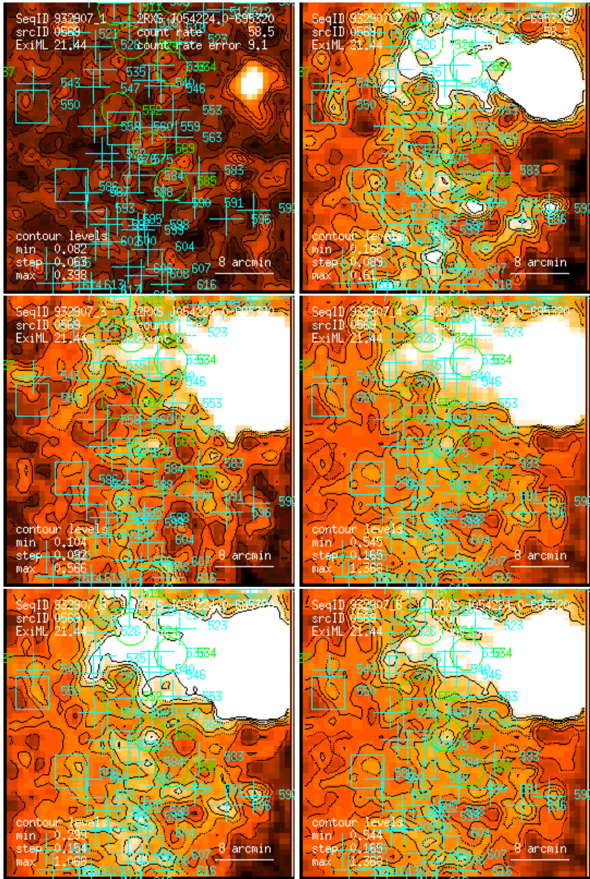
Figure 569: RASS 932907: detection 0569: band rate images, Gaussian filter: (1) PSPC channels 11 – 41, (2) 52 – 90, (3) 91 – 201, (4) 11 – 235, (5) 52 – 201, (6) 11 – 201. Broad band rates in counts/ks. Band rate contour levels in counts/ks/arcmin 2 .
