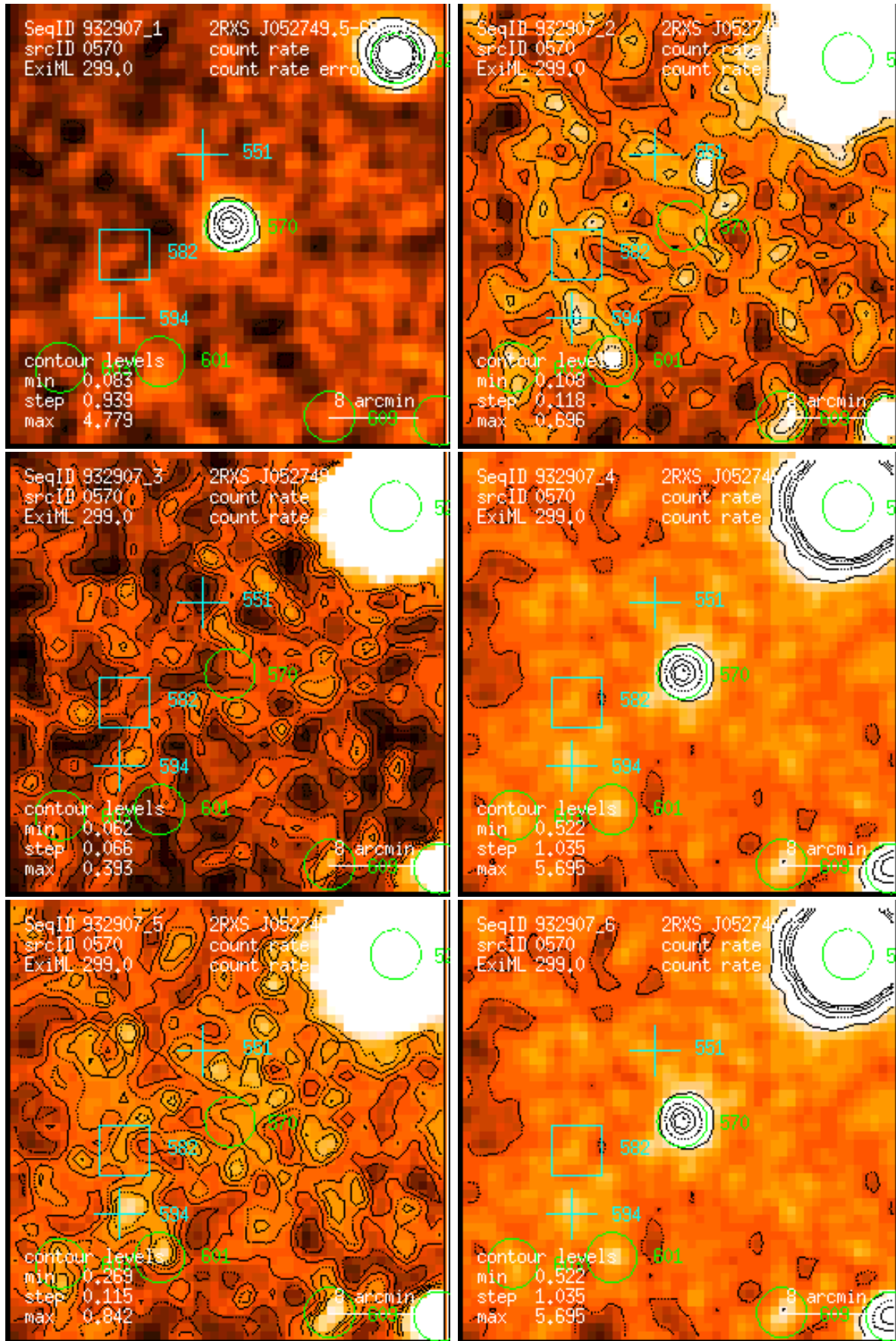
Figure 570: RASS 932907: detection 0570: band rate images, Gaussian filter: (1) PSPC channels 11 – 41, (2) 52 – 90, (3) 91 – 201, (4) 11 – 235, (5) 52 – 201, (6) 11 – 201. Broad band rates in counts/ks. Band rate contour levels in counts/ks/arcmin 2 .
