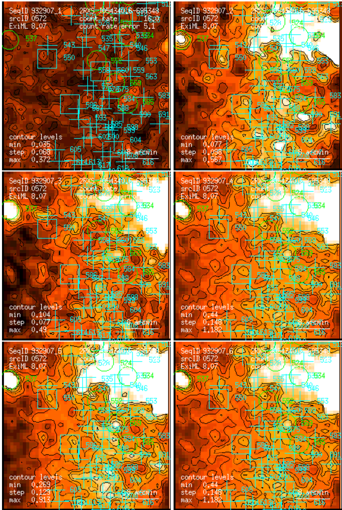
Figure 572: RASS 932907: detection 0572: band rate images, Gaussian filter: (1) PSPC channels 11 – 41, (2) 52 – 90, (3) 91 – 201, (4) 11 – 235, (5) 52 – 201, (6) 11 – 201. Broad band rates in counts/ks. Band rate contour levels in counts/ks/arcmin 2 .
