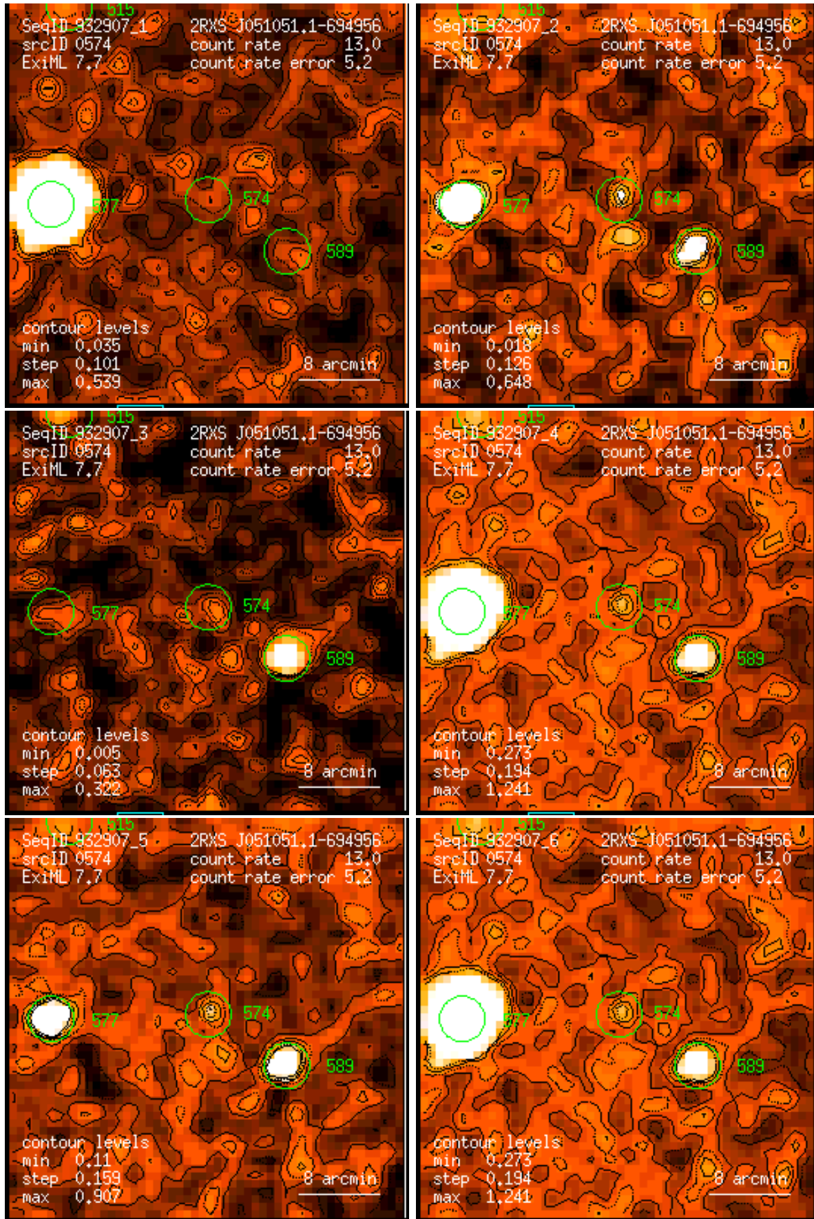
Figure 574: RASS 932907: detection 0574: band rate images, Gaussian filter: (1) PSPC channels 11 – 41, (2) 52 – 90, (3) 91 – 201, (4) 11 – 235, (5) 52 – 201, (6) 11 – 201. Broad band rates in counts/ks. Band rate contour levels in counts/ks/arcmin 2 .
