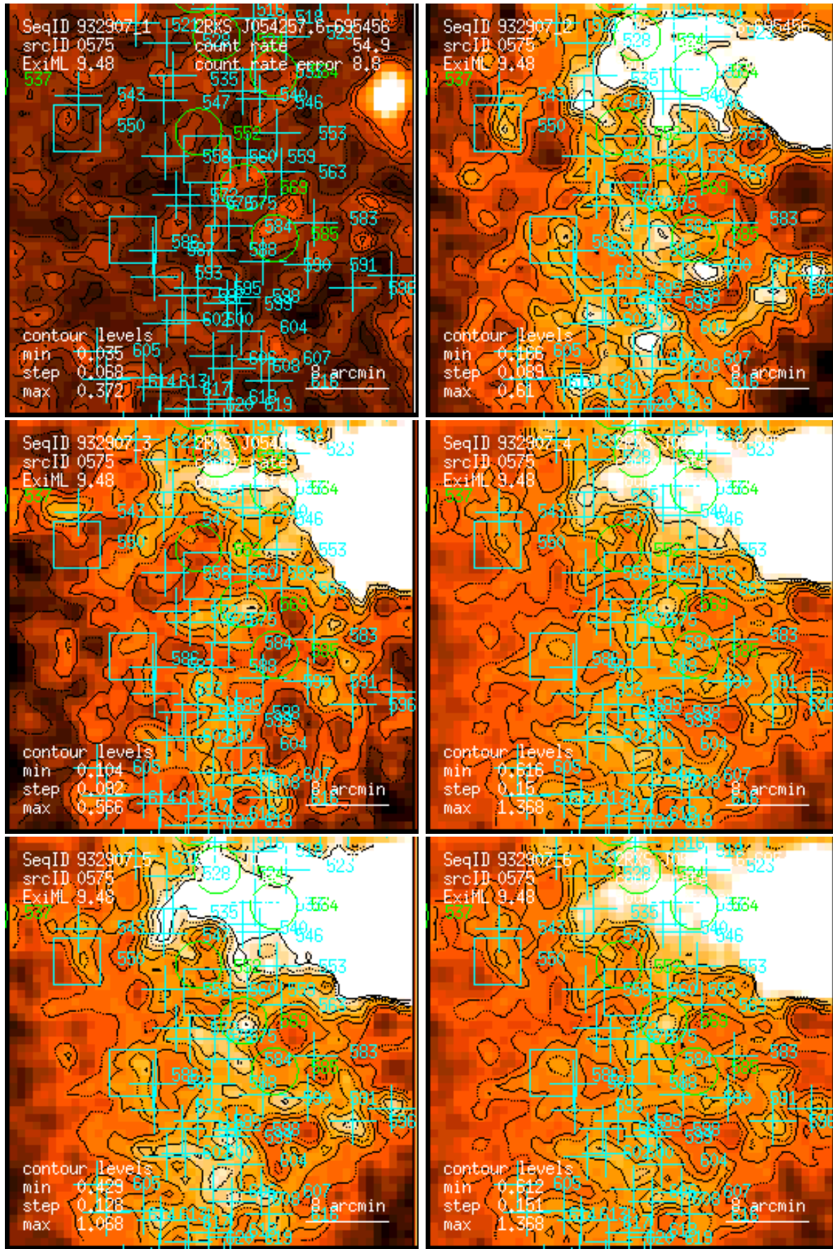
Figure 575: RASS 932907: detection 0575: band rate images, Gaussian filter: (1) PSPC channels 11 – 41, (2) 52 – 90, (3) 91 – 201, (4) 11 – 235, (5) 52 – 201, (6) 11 – 201. Broad band rates in counts/ks. Band rate contour levels in counts/ks/arcmin 2 .
