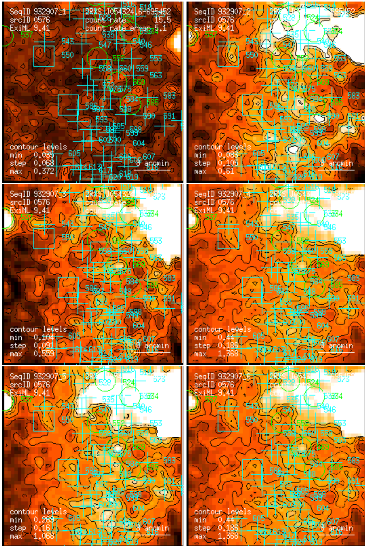
Figure 576: RASS 932907: detection 0576: band rate images, Gaussian filter: (1) PSPC channels 11 – 41, (2) 52 – 90, (3) 91 – 201, (4) 11 – 235, (5) 52 – 201, (6) 11 – 201. Broad band rates in counts/ks. Band rate contour levels in counts/ks/arcmin 2 .
