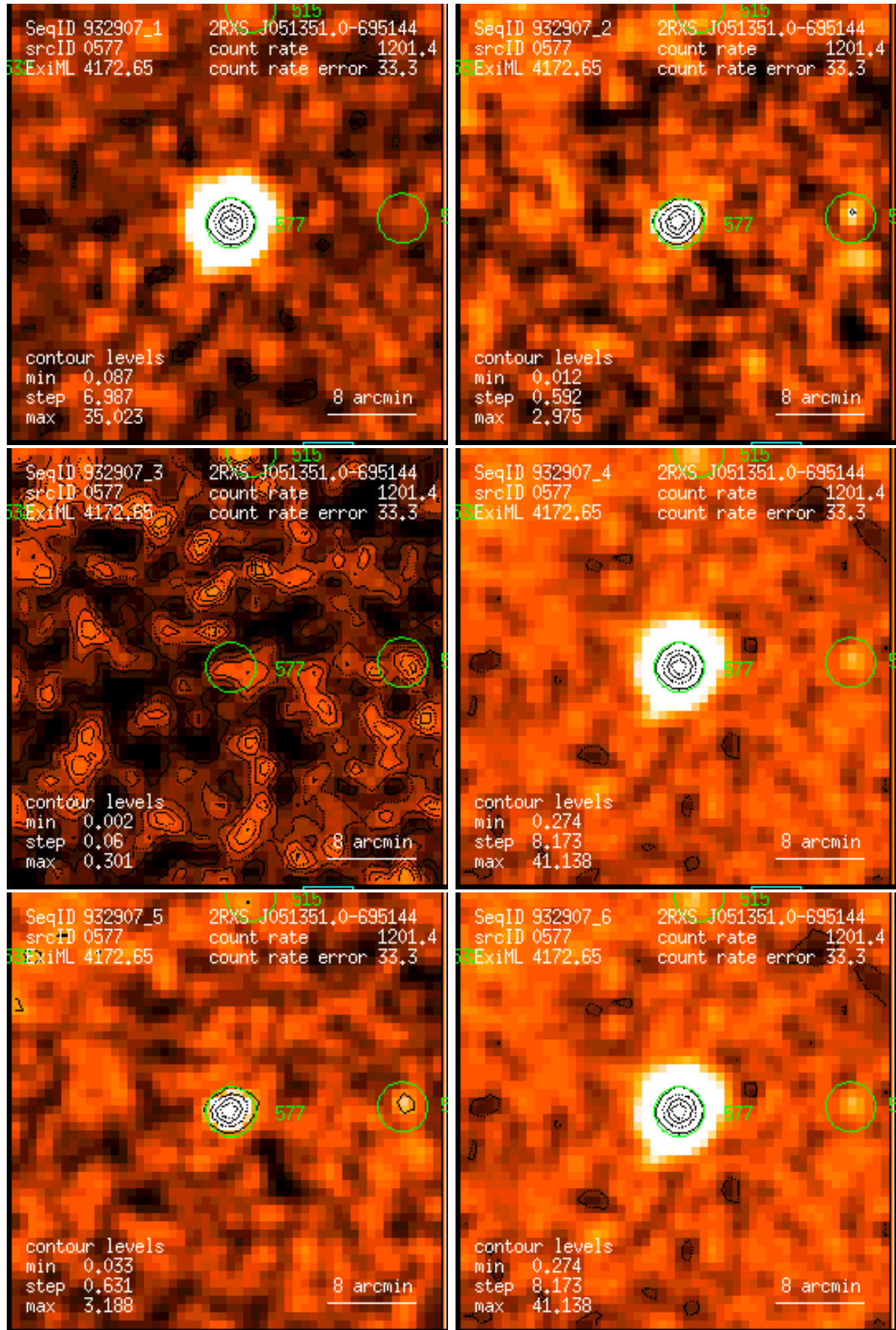
Figure 577: RASS 932907: detection 0577: band rate images, Gaussian filter: (1) PSPC channels 11 – 41, (2) 52 – 90, (3) 91 – 201, (4) 11 – 235, (5) 52 – 201, (6) 11 – 201. Broad band rates in counts/ks. Band rate contour levels in counts/ks/arcmin 2 .
