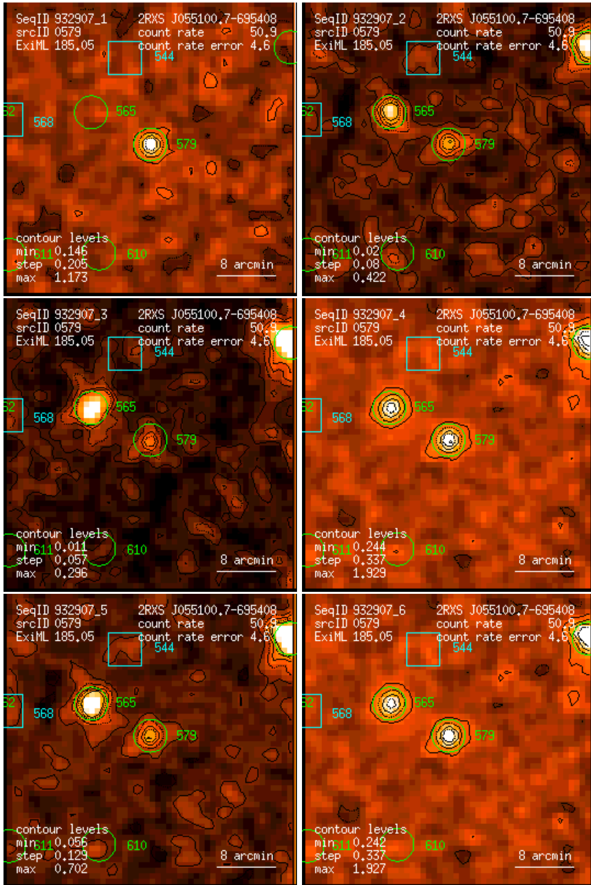
Figure 579: RASS 932907: detection 0579: band rate images, Gaussian filter: (1) PSPC channels 11 – 41, (2) 52 – 90, (3) 91 – 201, (4) 11 – 235, (5) 52 – 201, (6) 11 – 201. Broad band rates in counts/ks. Band rate contour levels in counts/ks/arcmin 2 .
