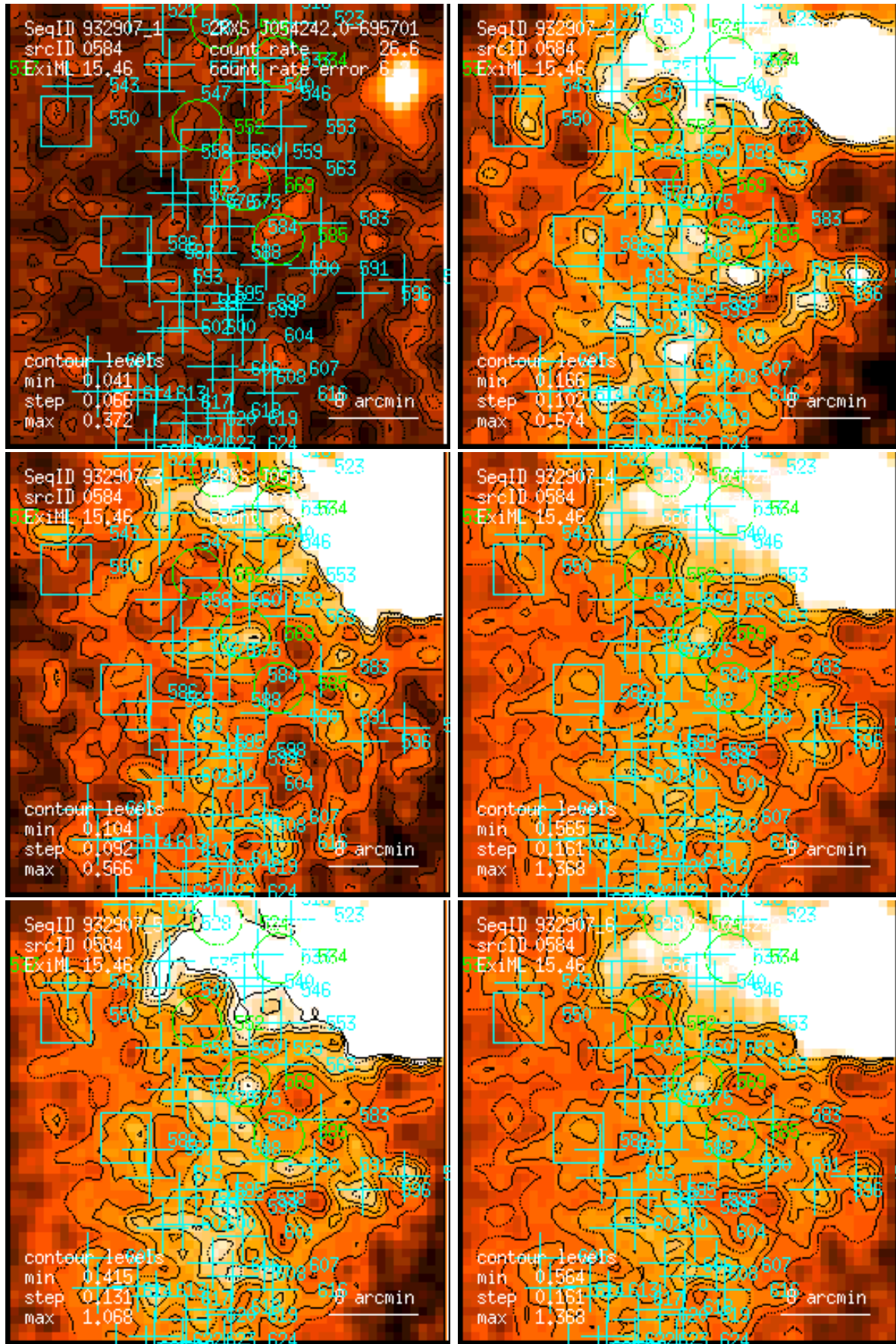
Figure 584: RASS 932907: detection 0584: band rate images, Gaussian filter: (1) PSPC channels 11 – 41, (2) 52 – 90, (3) 91 – 201, (4) 11 – 235, (5) 52 – 201, (6) 11 – 201. Broad band rates in counts/ks. Band rate contour levels in counts/ks/arcmin 2 .
