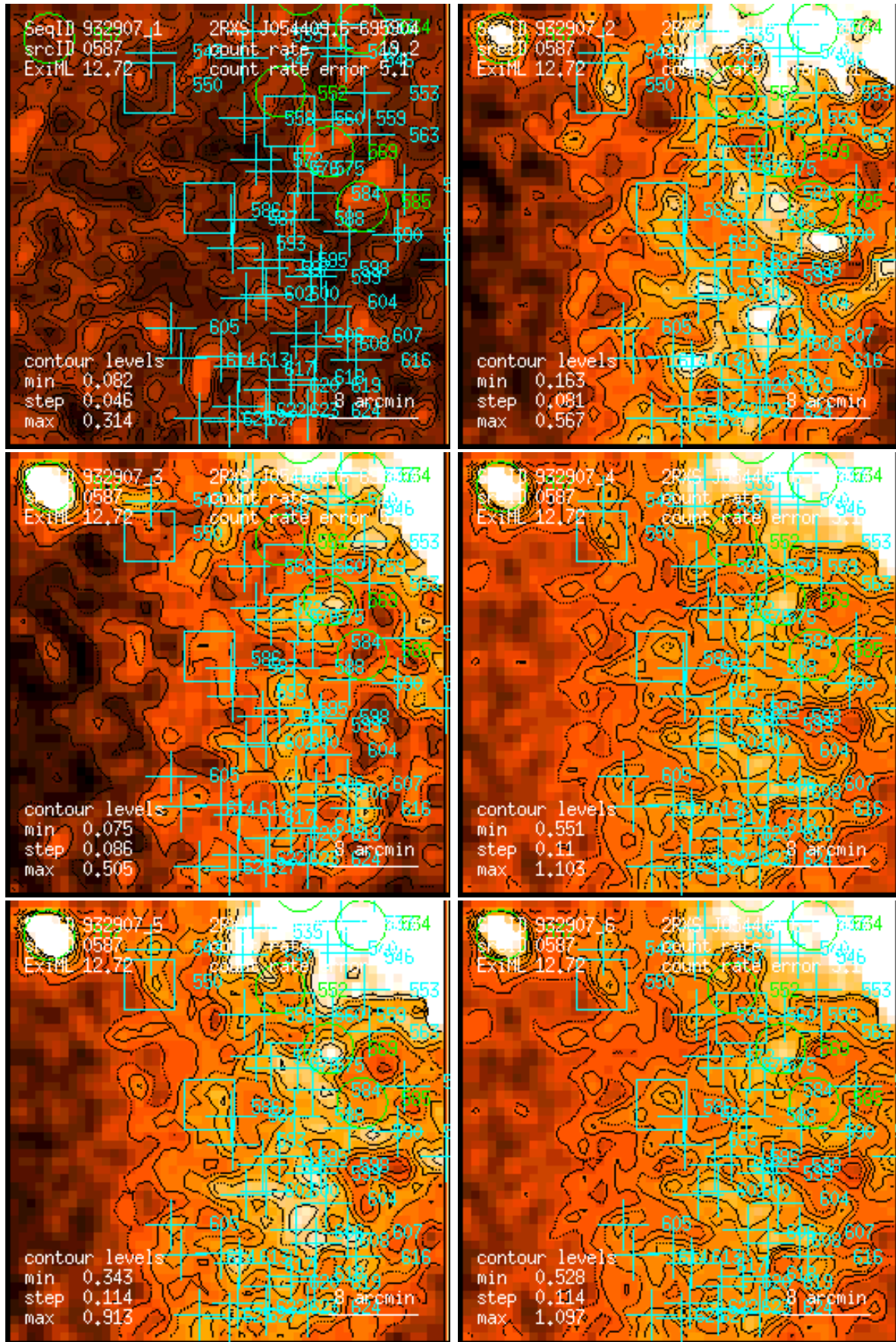
Figure 587: RASS 932907: detection 0587: band rate images, Gaussian filter: (1) PSPC channels 11 – 41, (2) 52 – 90, (3) 91 – 201, (4) 11 – 235, (5) 52 – 201, (6) 11 – 201. Broad band rates in counts/ks. Band rate contour levels in counts/ks/arcmin 2 .
