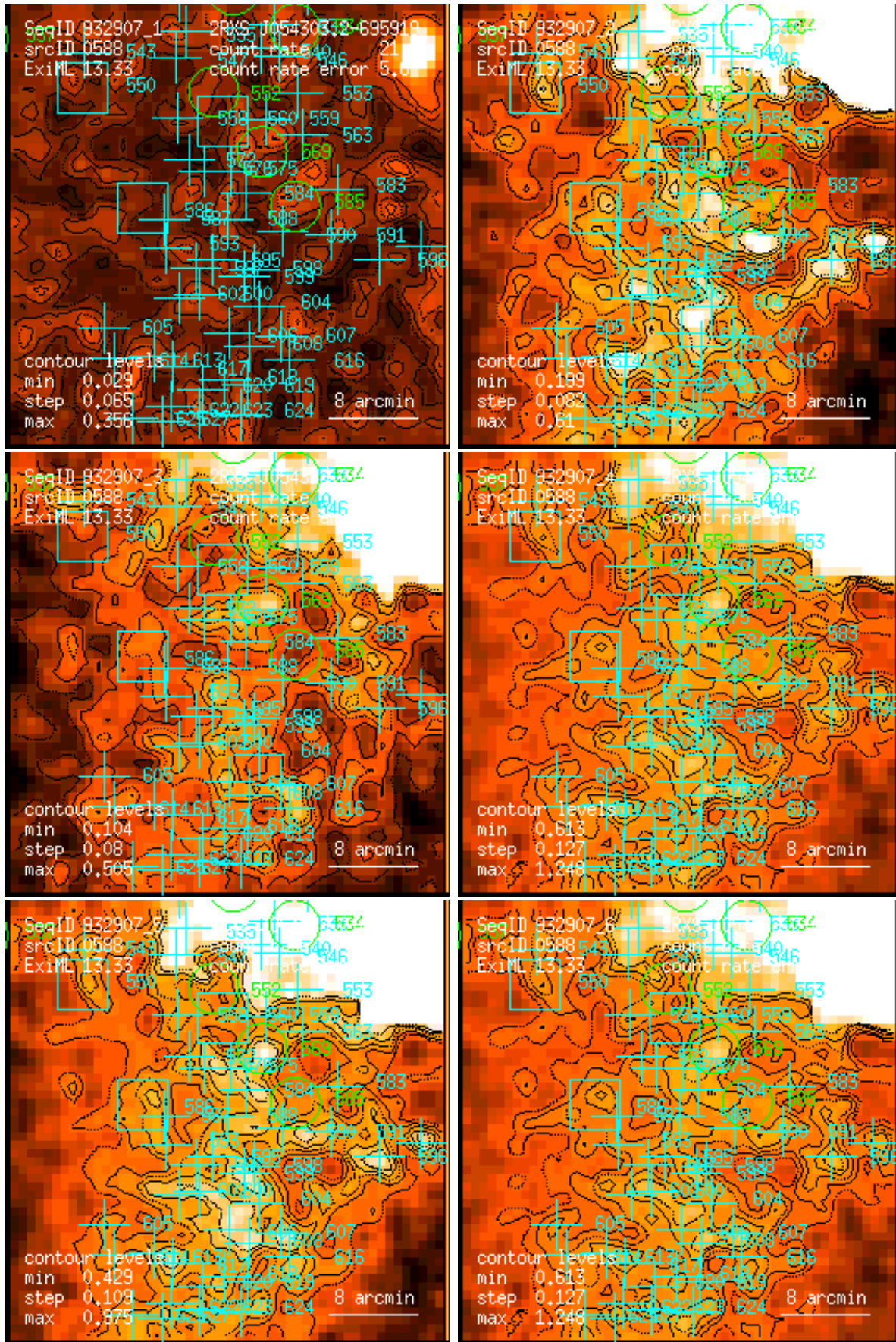
Figure 588: RASS 932907: detection 0588: band rate images, Gaussian filter: (1) PSPC channels 11 – 41, (2) 52 – 90, (3) 91 – 201, (4) 11 – 235, (5) 52 – 201, (6) 11 – 201. Broad band rates in counts/ks. Band rate contour levels in counts/ks/arcmin 2 .
