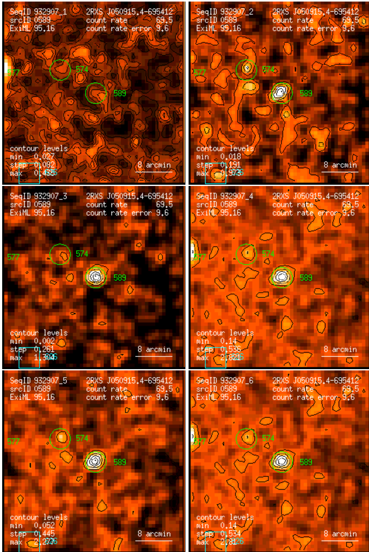
Figure 589: RASS 932907: detection 0589: band rate images, Gaussian filter: (1) PSPC channels 11 – 41, (2) 52 – 90, (3) 91 – 201, (4) 11 – 235, (5) 52 – 201, (6) 11 – 201. Broad band rates in counts/ks. Band rate contour levels in counts/ks/arcmin 2 .
