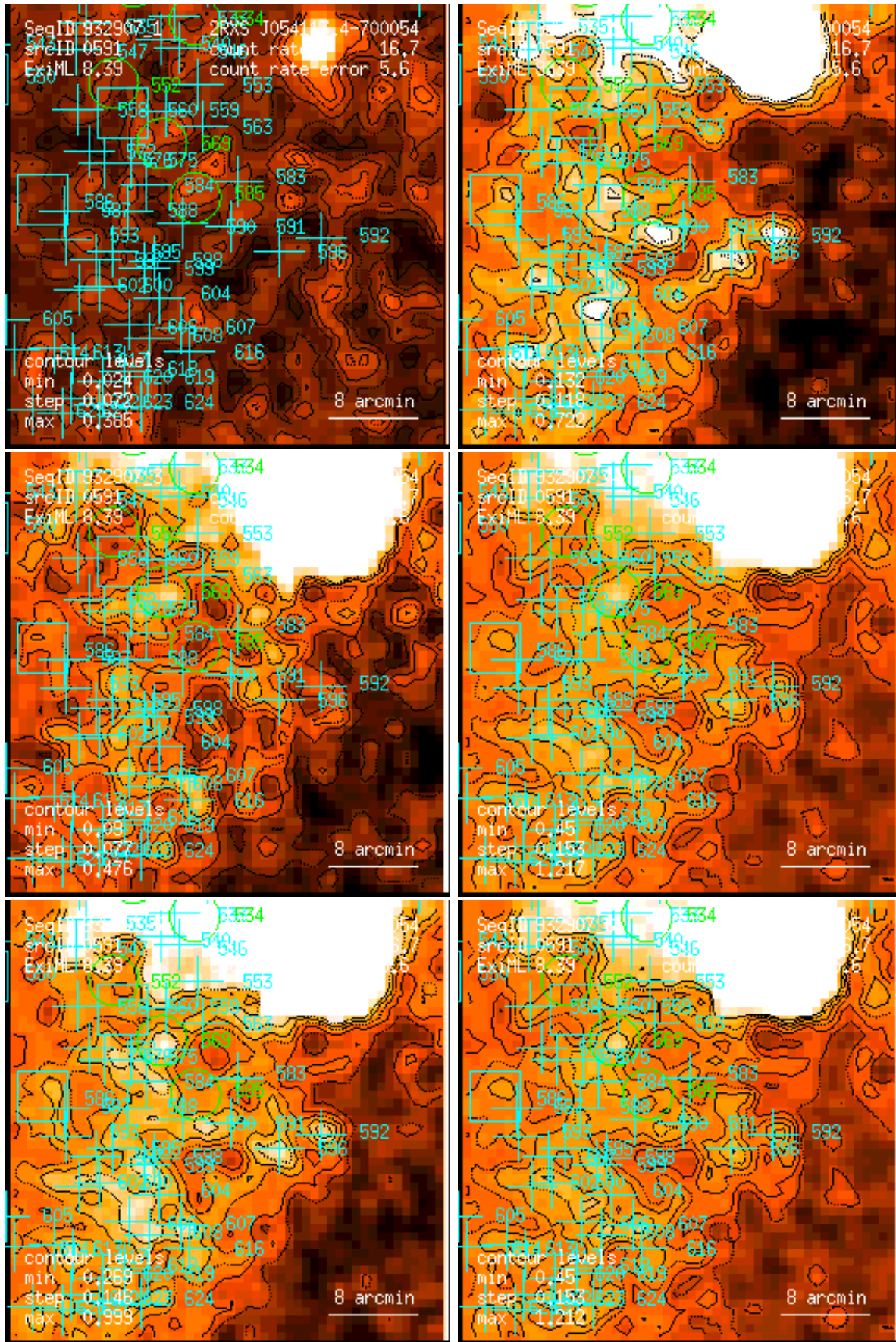
Figure 591: RASS 932907: detection 0591: band rate images, Gaussian filter: (1) PSPC channels 11 – 41, (2) 52 – 90, (3) 91 – 201, (4) 11 – 235, (5) 52 – 201, (6) 11 – 201. Broad band rates in counts/ks. Band rate contour levels in counts/ks/arcmin 2 .
