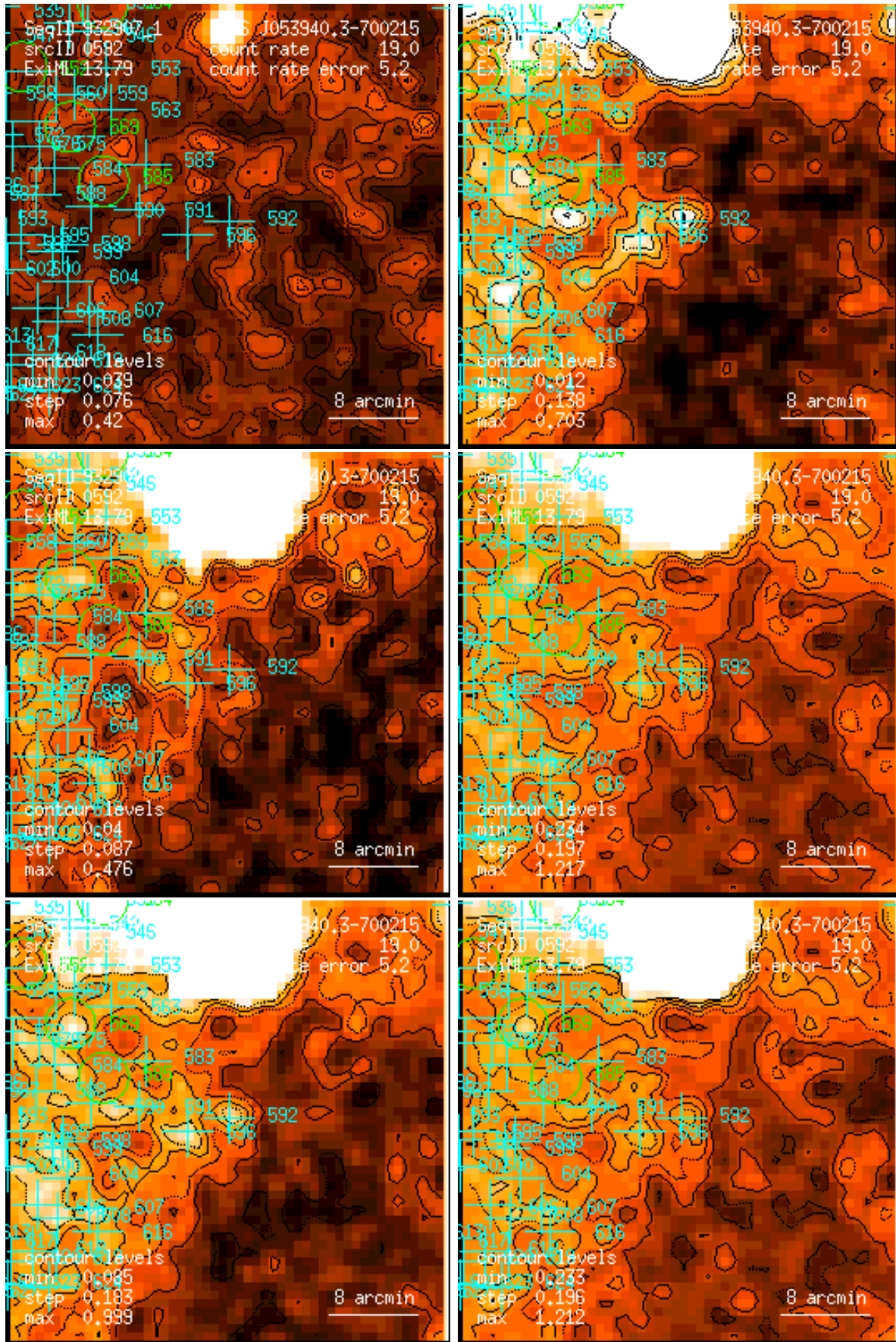
Figure 592: RASS 932907: detection 0592: band rate images, Gaussian filter: (1) PSPC channels 11 – 41, (2) 52 – 90, (3) 91 – 201, (4) 11 – 235, (5) 52 – 201, (6) 11 – 201. Broad band rates in counts/ks. Band rate contour levels in counts/ks/arcmin 2 .
