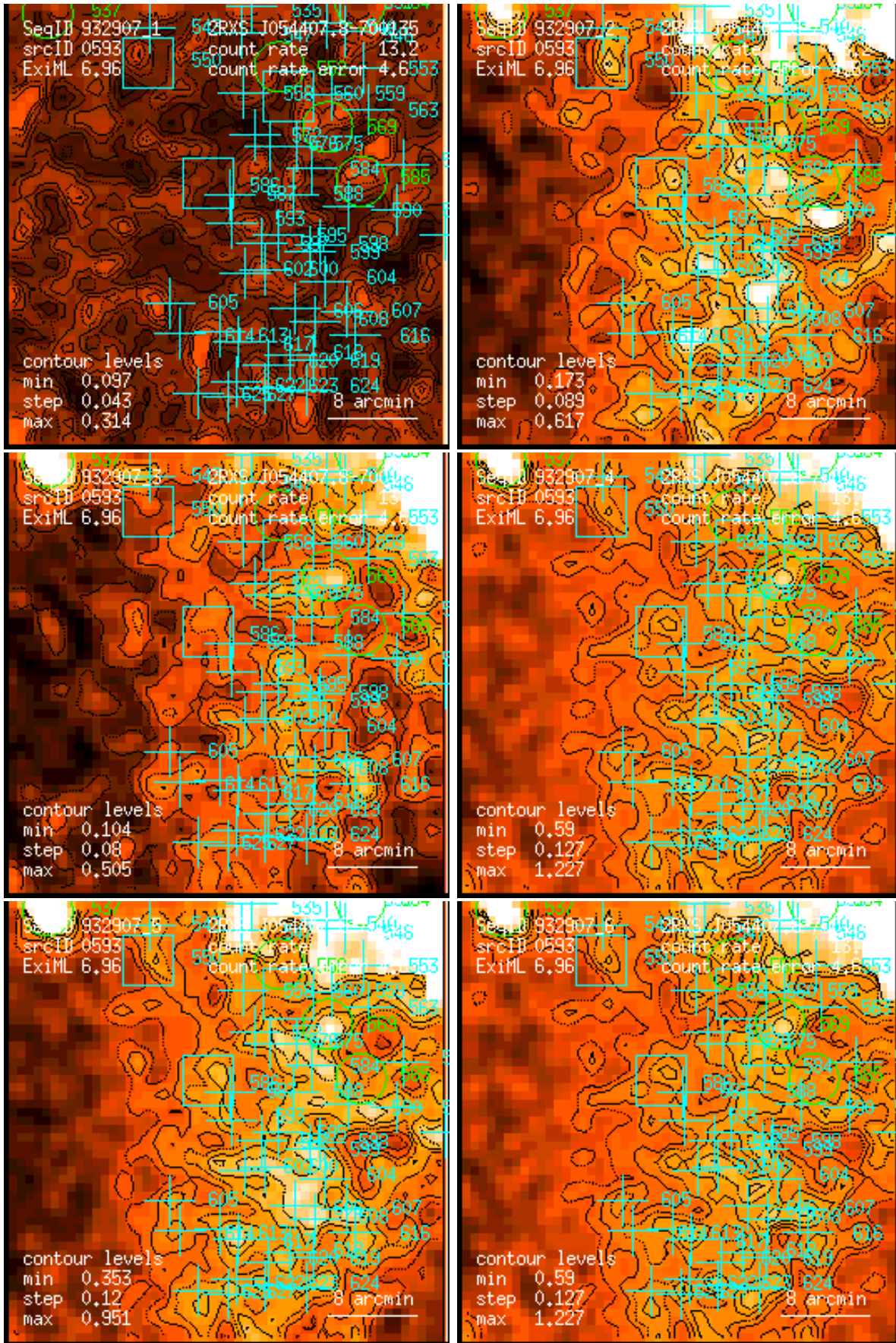
Figure 593: RASS 932907: detection 0593: band rate images, Gaussian filter: (1) PSPC channels 11 – 41, (2) 52 – 90, (3) 91 – 201, (4) 11 – 235, (5) 52 – 201, (6) 11 – 201. Broad band rates in counts/ks. Band rate contour levels in counts/ks/arcmin 2 .
