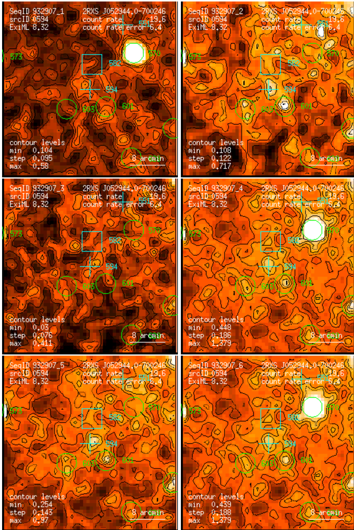
Figure 594: RASS 932907: detection 0594: band rate images, Gaussian filter: (1) PSPC channels 11 – 41, (2) 52 – 90, (3) 91 – 201, (4) 11 – 235, (5) 52 – 201, (6) 11 – 201. Broad band rates in counts/ks. Band rate contour levels in counts/ks/arcmin 2 .
