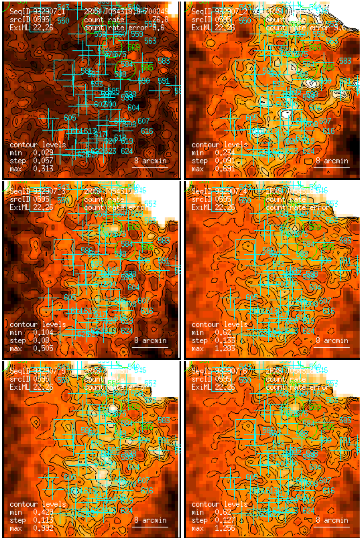
Figure 595: RASS 932907: detection 0595: band rate images, Gaussian filter: (1) PSPC channels 11 – 41, (2) 52 – 90, (3) 91 – 201, (4) 11 – 235, (5) 52 – 201, (6) 11 – 201. Broad band rates in counts/ks. Band rate contour levels in counts/ks/arcmin 2 .
