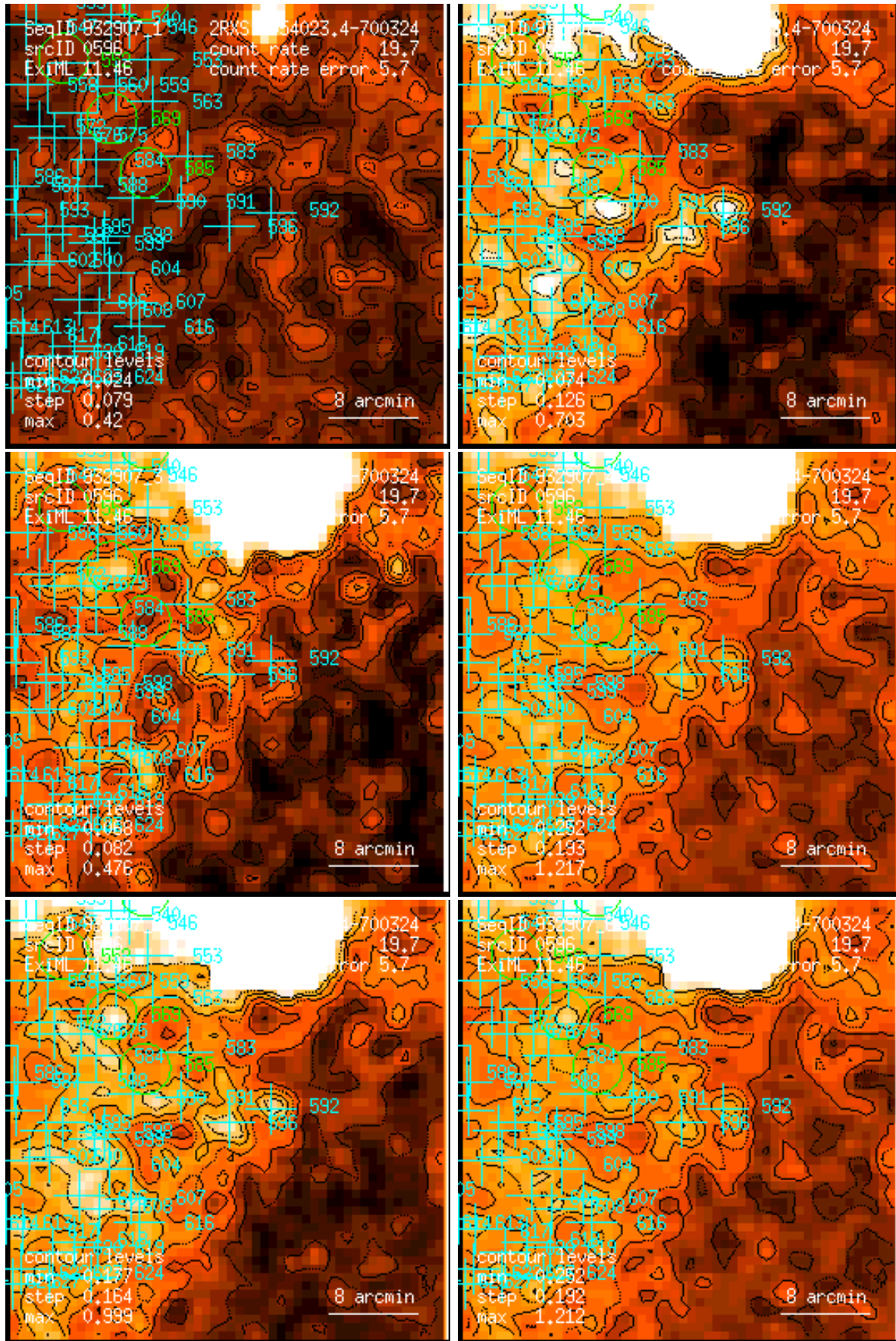
Figure 596: RASS 932907: detection 0596: band rate images, Gaussian filter: (1) PSPC channels 11 – 41, (2) 52 – 90, (3) 91 – 201, (4) 11 – 235, (5) 52 – 201, (6) 11 – 201. Broad band rates in counts/ks. Band rate contour levels in counts/ks/arcmin 2 .
