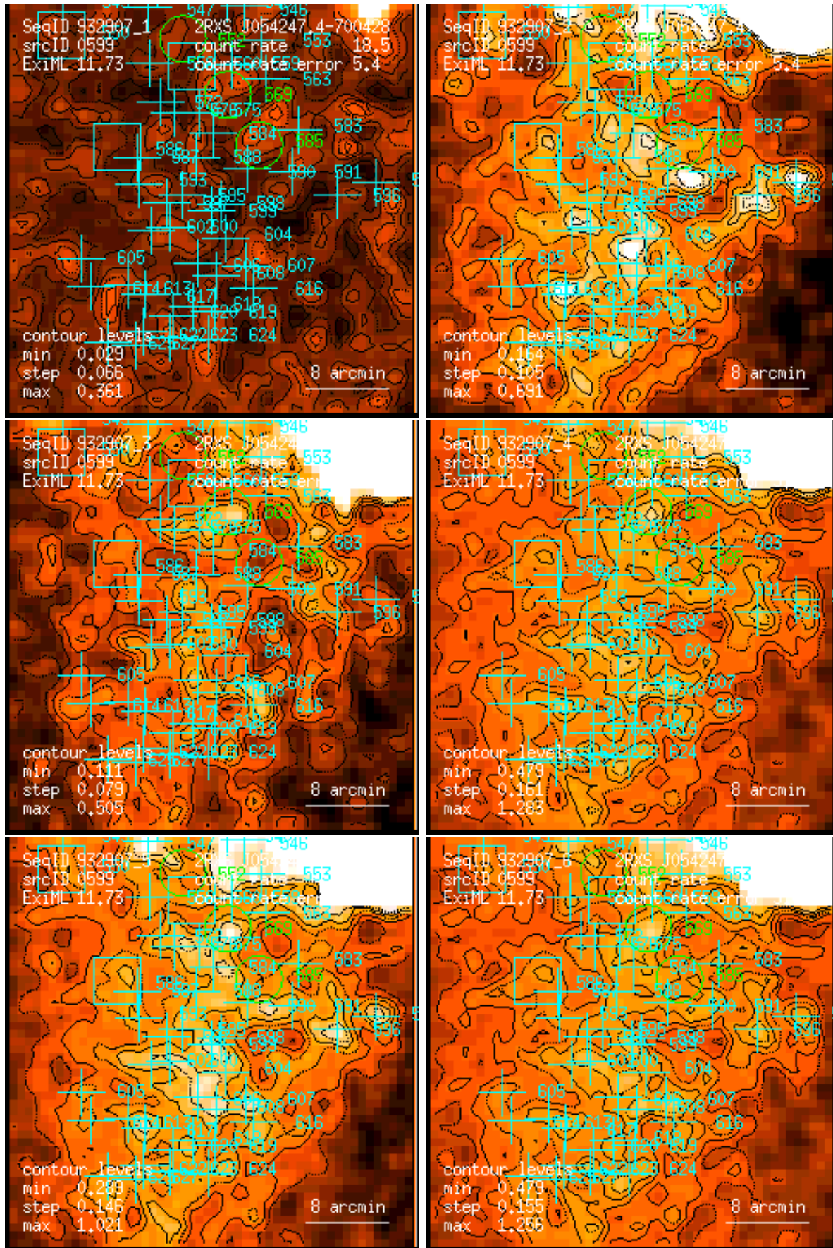
Figure 599: RASS 932907: detection 0599: band rate images, Gaussian filter: (1) PSPC channels 11 – 41, (2) 52 – 90, (3) 91 – 201, (4) 11 – 235, (5) 52 – 201, (6) 11 – 201. Broad band rates in counts/ks. Band rate contour levels in counts/ks/arcmin 2 .
