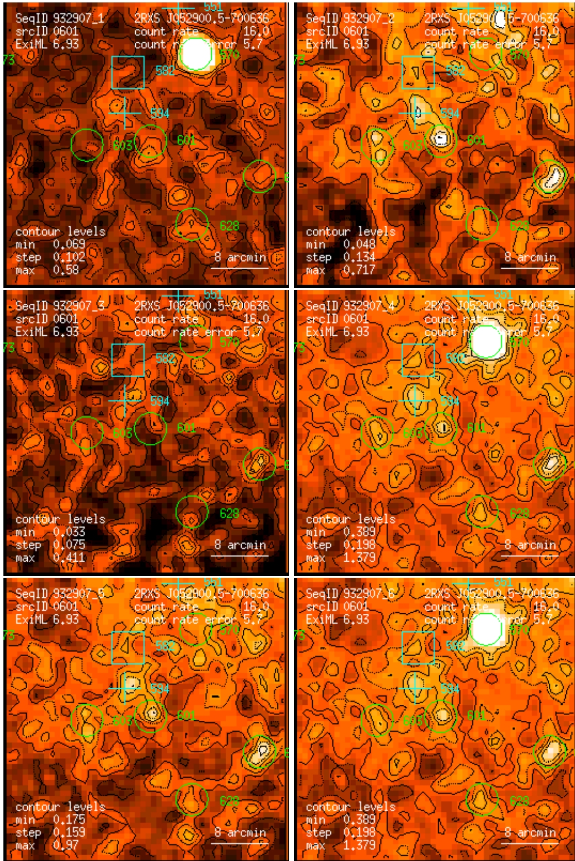
Figure 601: RASS 932907: detection 0601: band rate images, Gaussian filter: (1) PSPC channels 11 – 41, (2) 52 – 90, (3) 91 – 201, (4) 11 – 235, (5) 52 – 201, (6) 11 – 201. Broad band rates in counts/ks. Band rate contour levels in counts/ks/arcmin 2 .
