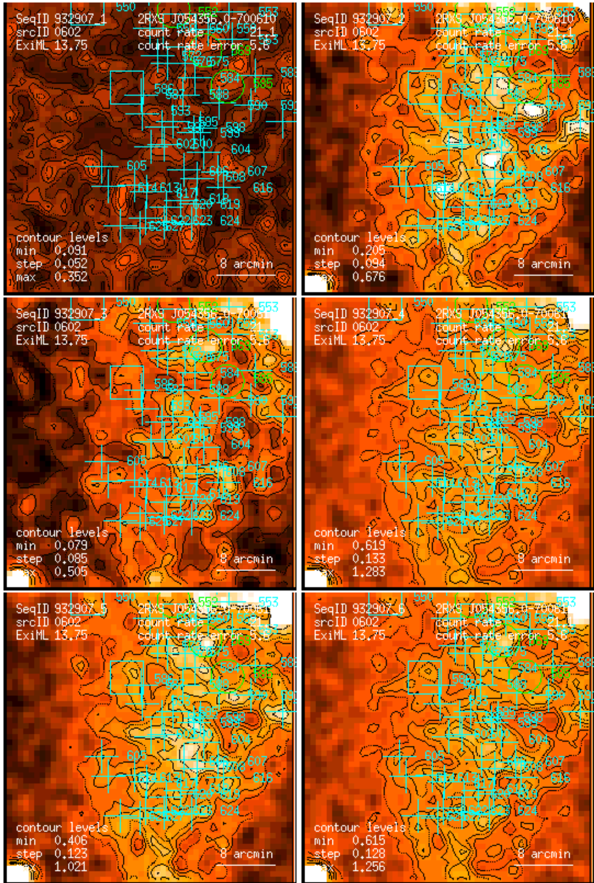
Figure 602: RASS 932907: detection 0602: band rate images, Gaussian filter: (1) PSPC channels 11 – 41, (2) 52 – 90, (3) 91 – 201, (4) 11 – 235, (5) 52 – 201, (6) 11 – 201. Broad band rates in counts/ks. Band rate contour levels in counts/ks/arcmin 2 .
