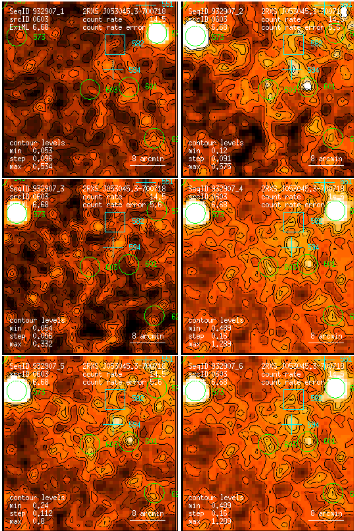
Figure 603: RASS 932907: detection 0603: band rate images, Gaussian filter: (1) PSPC channels 11 – 41, (2) 52 – 90, (3) 91 – 201, (4) 11 – 235, (5) 52 – 201, (6) 11 – 201. Broad band rates in counts/ks. Band rate contour levels in counts/ks/arcmin 2 .
