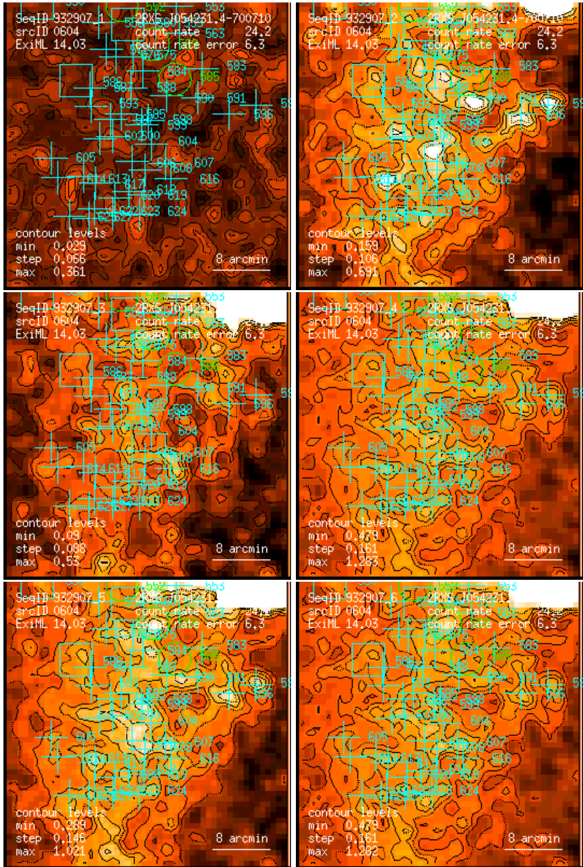
Figure 604: RASS 932907: detection 0604: band rate images, Gaussian filter: (1) PSPC channels 11 – 41, (2) 52 – 90, (3) 91 – 201, (4) 11 – 235, (5) 52 – 201, (6) 11 – 201. Broad band rates in counts/ks. Band rate contour levels in counts/ks/arcmin 2 .
