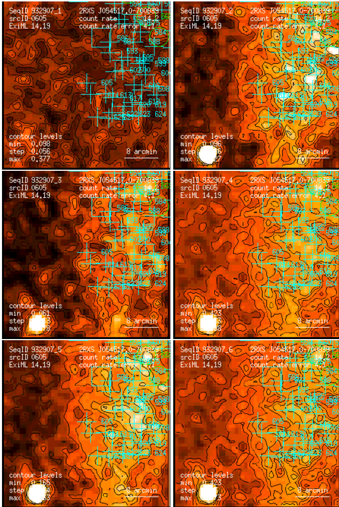
Figure 605: RASS 932907: detection 0605: band rate images, Gaussian filter: (1) PSPC channels 11 – 41, (2) 52 – 90, (3) 91 – 201, (4) 11 – 235, (5) 52 – 201, (6) 11 – 201. Broad band rates in counts/ks. Band rate contour levels in counts/ks/arcmin 2 .
