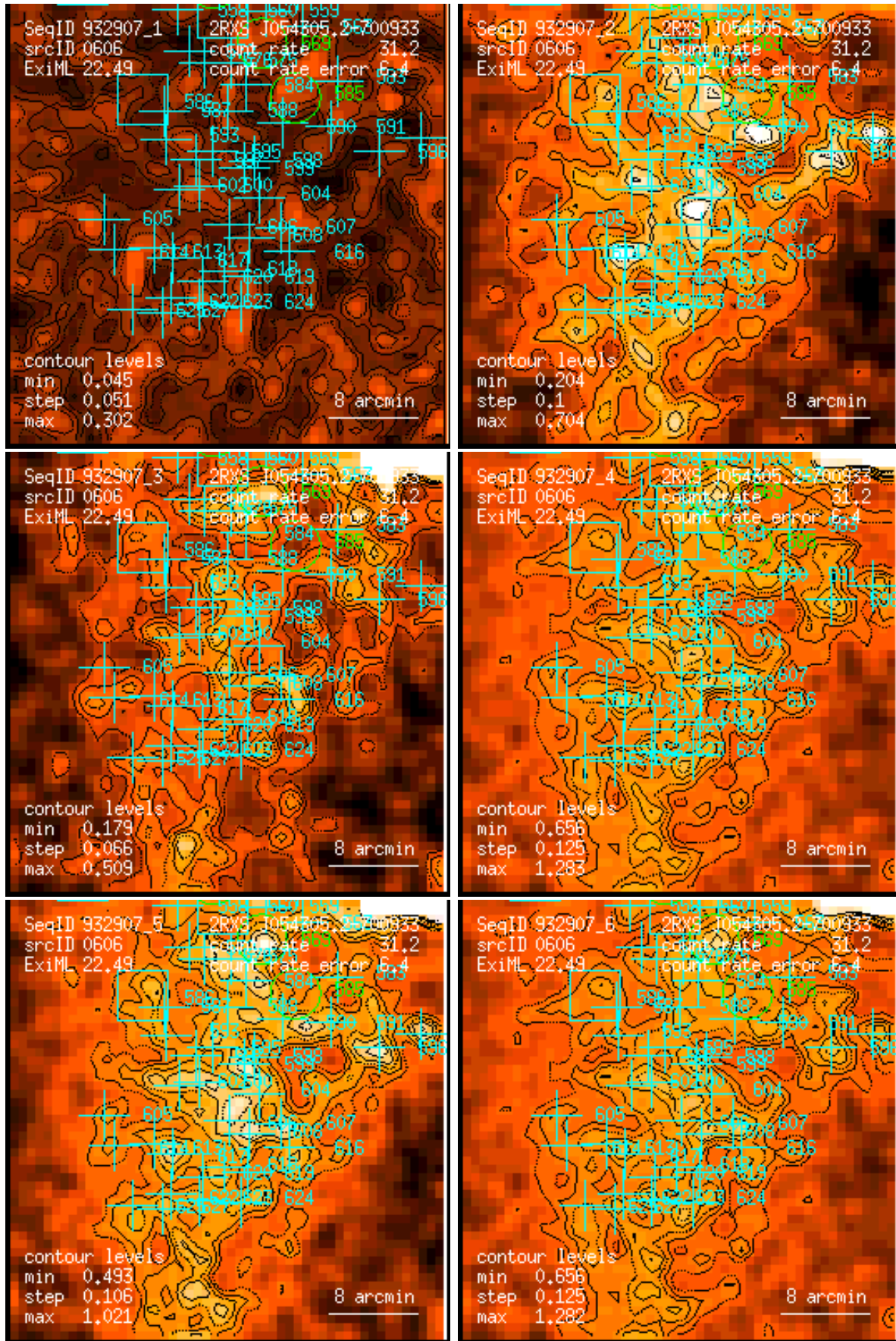
Figure 606: RASS 932907: detection 0606: band rate images, Gaussian filter: (1) PSPC channels 11 – 41, (2) 52 – 90, (3) 91 – 201, (4) 11 – 235, (5) 52 – 201, (6) 11 – 201. Broad band rates in counts/ks. Band rate contour levels in counts/ks/arcmin 2 .
