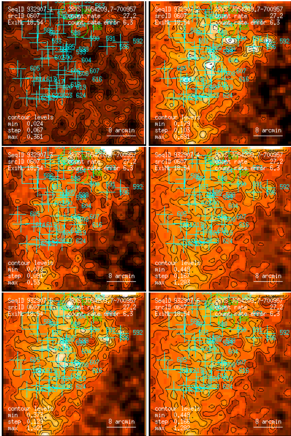
Figure 607: RASS 932907: detection 0607: band rate images, Gaussian filter: (1) PSPC channels 11 – 41, (2) 52 – 90, (3) 91 – 201, (4) 11 – 235, (5) 52 – 201, (6) 11 – 201. Broad band rates in counts/ks. Band rate contour levels in counts/ks/arcmin 2 .
