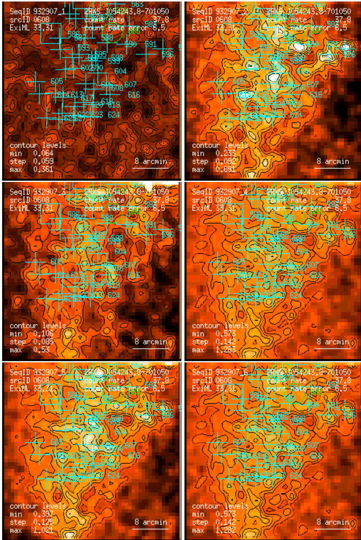
Figure 608: RASS 932907: detection 0608: band rate images, Gaussian filter: (1) PSPC channels 11 – 41, (2) 52 – 90, (3) 91 – 201, (4) 11 – 235, (5) 52 – 201, (6) 11 – 201. Broad band rates in counts/ks. Band rate contour levels in counts/ks/arcmin 2 .
