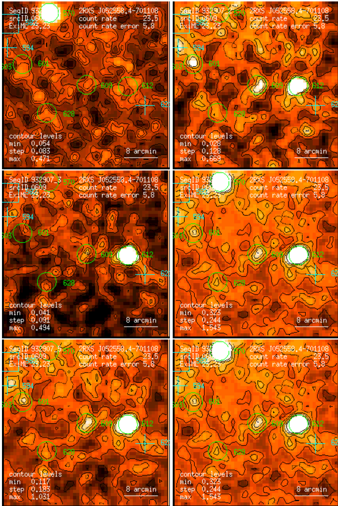
Figure 609: RASS 932907: detection 0609: band rate images, Gaussian filter: (1) PSPC channels 11 – 41, (2) 52 – 90, (3) 91 – 201, (4) 11 – 235, (5) 52 – 201, (6) 11 – 201. Broad band rates in counts/ks. Band rate contour levels in counts/ks/arcmin 2 .
