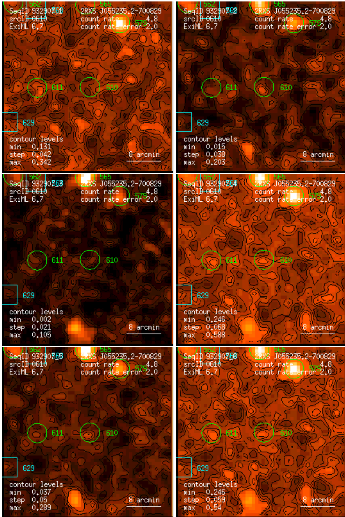
Figure 610: RASS 932907: detection 0610: band rate images, Gaussian filter: (1) PSPC channels 11 – 41, (2) 52 – 90, (3) 91 – 201, (4) 11 – 235, (5) 52 – 201, (6) 11 – 201. Broad band rates in counts/ks. Band rate contour levels in counts/ks/arcmin 2 .
