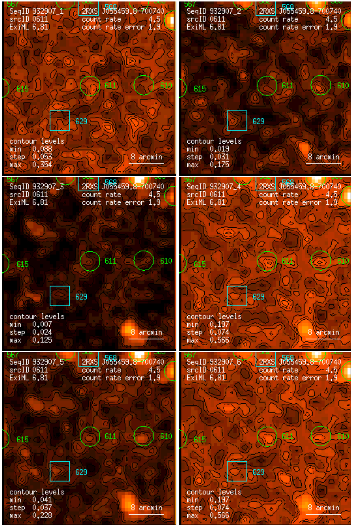
Figure 611: RASS 932907: detection 0611: band rate images, Gaussian filter: (1) PSPC channels 11 – 41, (2) 52 – 90, (3) 91 – 201, (4) 11 – 235, (5) 52 – 201, (6) 11 – 201. Broad band rates in counts/ks. Band rate contour levels in counts/ks/arcmin 2 .
