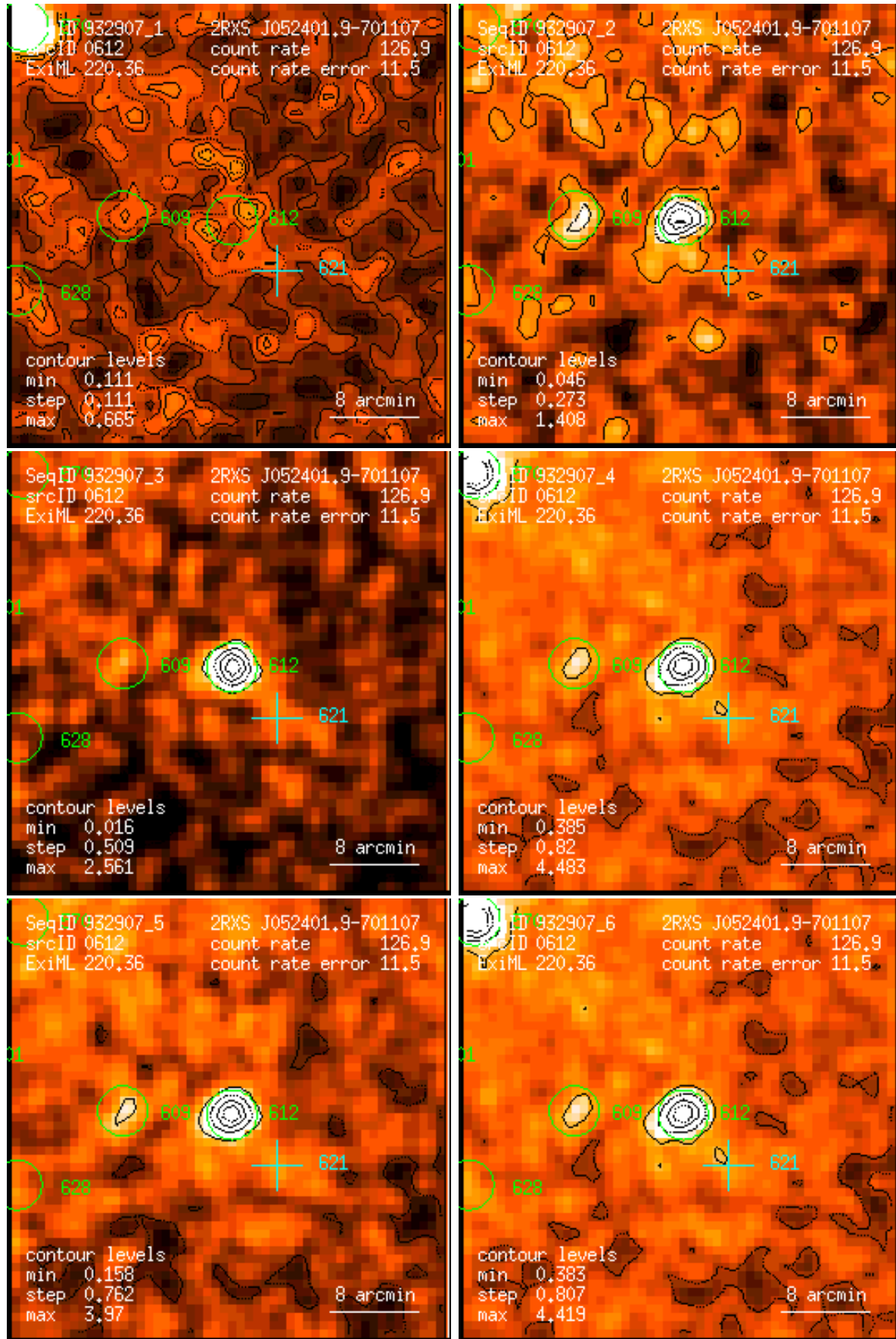
Figure 612: RASS 932907: detection 0612: band rate images, Gaussian filter: (1) PSPC channels 11 – 41, (2) 52 – 90, (3) 91 – 201, (4) 11 – 235, (5) 52 – 201, (6) 11 – 201. Broad band rates in counts/ks. Band rate contour levels in counts/ks/arcmin 2 .
