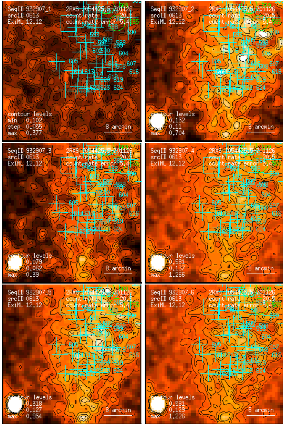
Figure 613: RASS 932907: detection 0613: band rate images, Gaussian filter: (1) PSPC channels 11 – 41, (2) 52 – 90, (3) 91 – 201, (4) 11 – 235, (5) 52 – 201, (6) 11 – 201. Broad band rates in counts/ks. Band rate contour levels in counts/ks/arcmin 2 .
