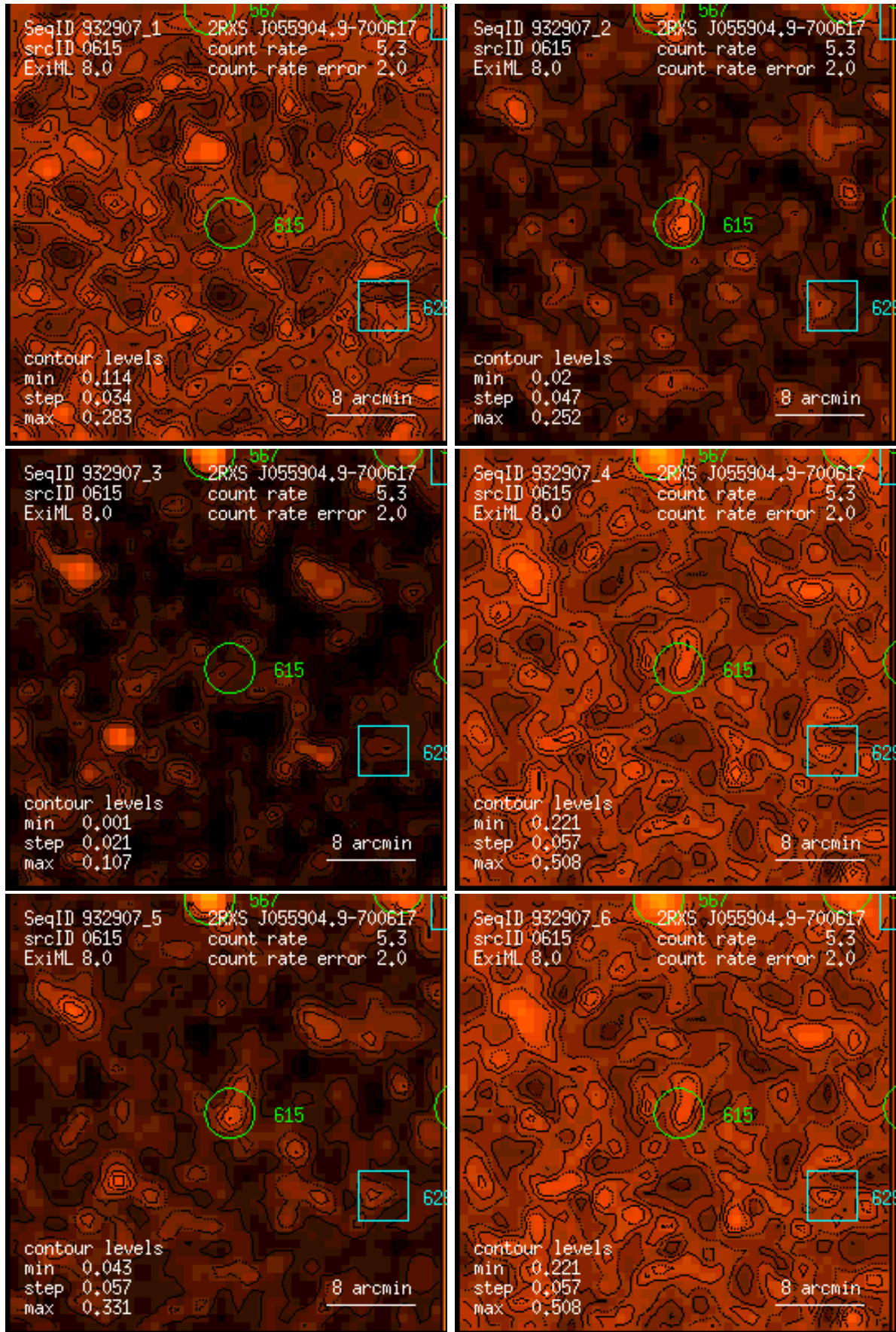
Figure 615: RASS 932907: detection 0615: band rate images, Gaussian filter: (1) PSPC channels 11 – 41, (2) 52 – 90, (3) 91 – 201, (4) 11 – 235, (5) 52 – 201, (6) 11 – 201. Broad band rates in counts/ks. Band rate contour levels in counts/ks/arcmin 2 .
