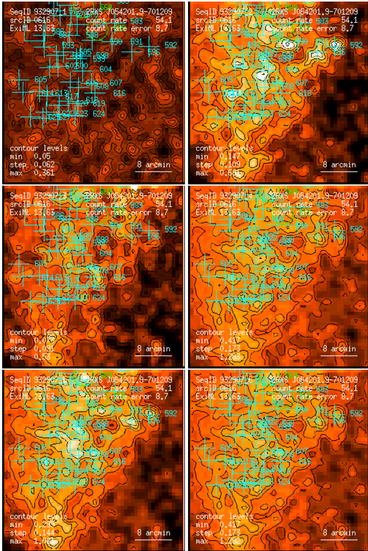
Figure 616: RASS 932907: detection 0616: band rate images, Gaussian filter: (1) PSPC channels 11 – 41, (2) 52 – 90, (3) 91 – 201, (4) 11 – 235, (5) 52 – 201, (6) 11 – 201. Broad band rates in counts/ks. Band rate contour levels in counts/ks/arcmin 2 .
