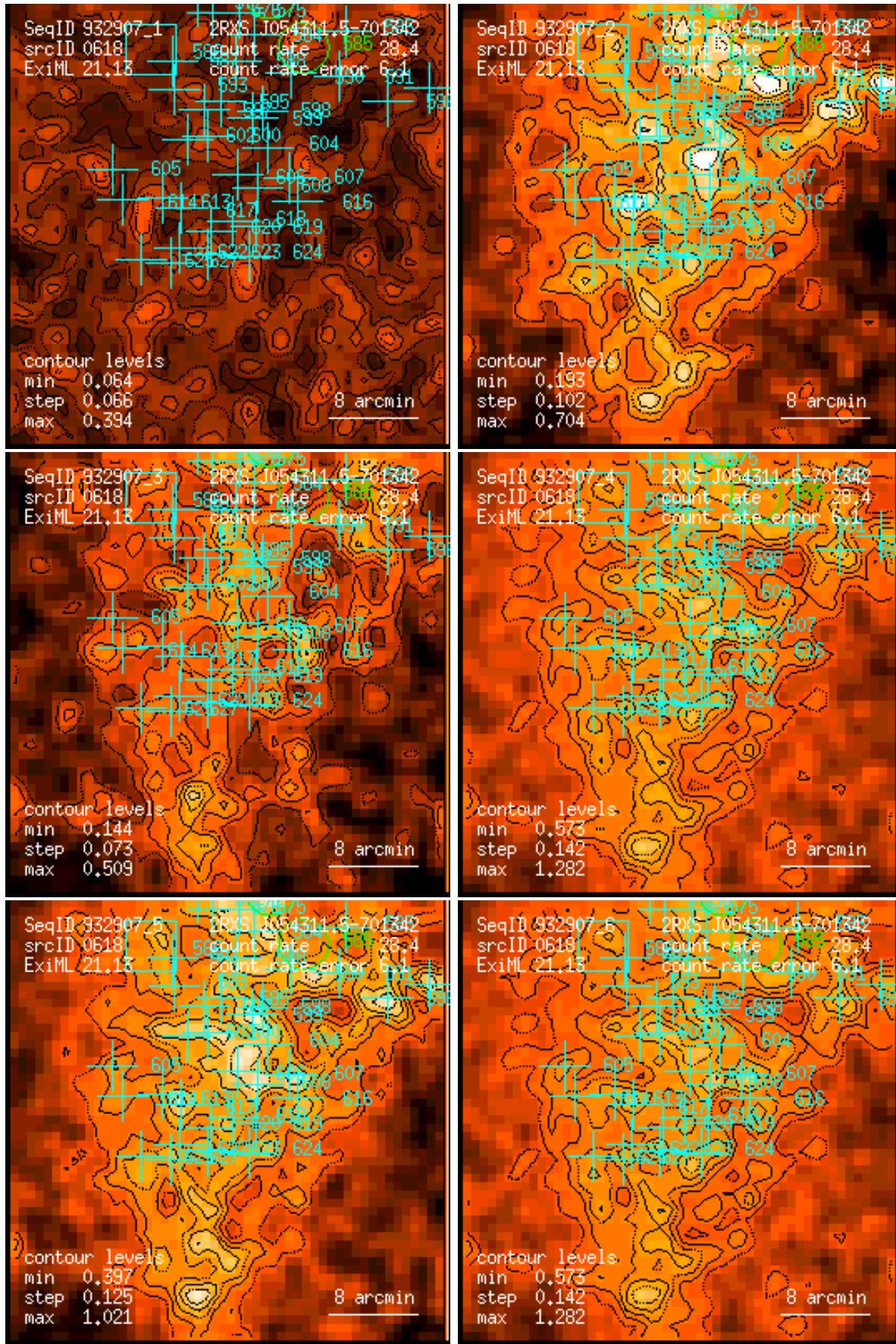
Figure 618: RASS 932907: detection 0618: band rate images, Gaussian filter: (1) PSPC channels 11 – 41, (2) 52 – 90, (3) 91 – 201, (4) 11 – 235, (5) 52 – 201, (6) 11 – 201. Broad band rates in counts/ks. Band rate contour levels in counts/ks/arcmin 2 .
