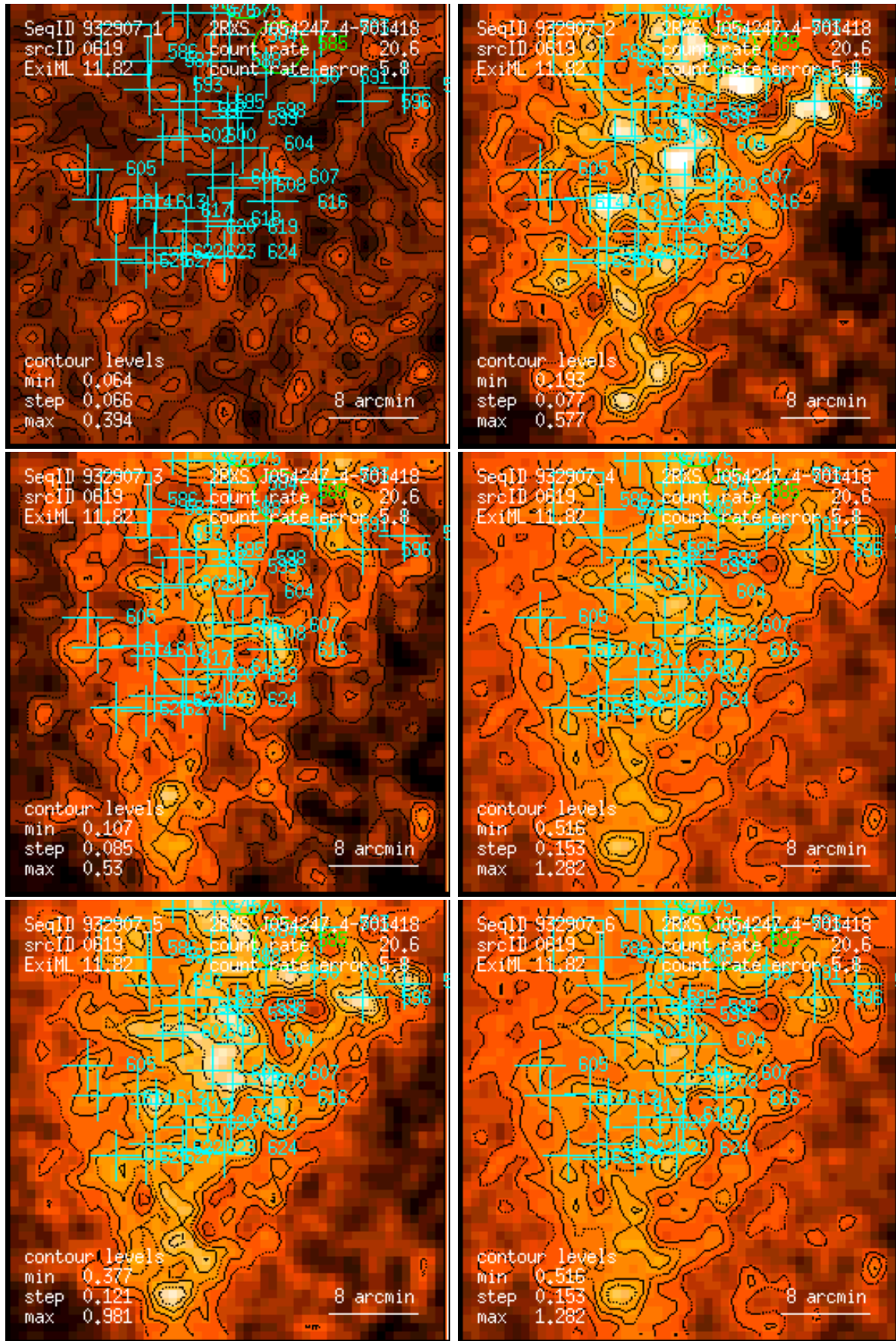
Figure 619: RASS 932907: detection 0619: band rate images, Gaussian filter: (1) PSPC channels 11 – 41, (2) 52 – 90, (3) 91 – 201, (4) 11 – 235, (5) 52 – 201, (6) 11 – 201. Broad band rates in counts/ks. Band rate contour levels in counts/ks/arcmin 2 .
