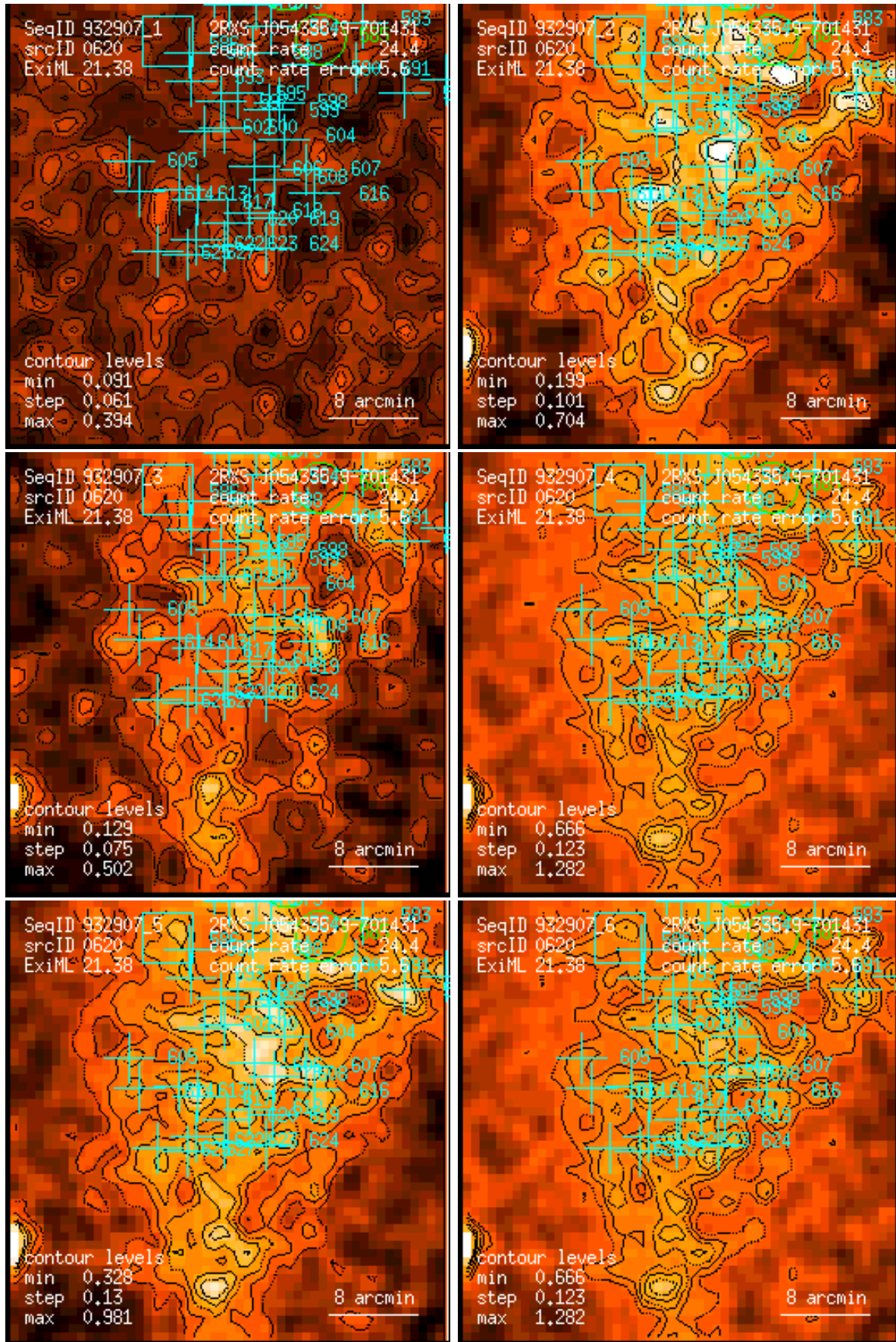
Figure 620: RASS 932907: detection 0620: band rate images, Gaussian filter: (1) PSPC channels 11 – 41, (2) 52 – 90, (3) 91 – 201, (4) 11 – 235, (5) 52 – 201, (6) 11 – 201. Broad band rates in counts/ks. Band rate contour levels in counts/ks/arcmin 2 .
