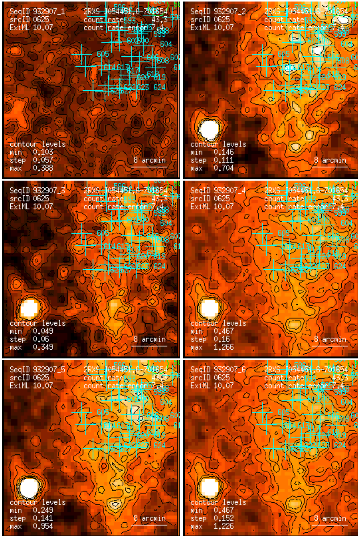
Figure 625: RASS 932907: detection 0625: band rate images, Gaussian filter: (1) PSPC channels 11 – 41, (2) 52 – 90, (3) 91 – 201, (4) 11 – 235, (5) 52 – 201, (6) 11 – 201. Broad band rates in counts/ks. Band rate contour levels in counts/ks/arcmin 2 .
