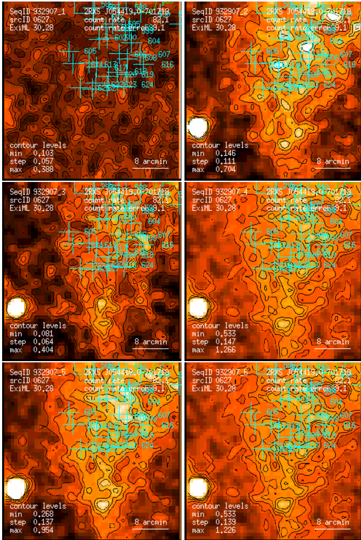
Figure 627: RASS 932907: detection 0627: band rate images, Gaussian filter: (1) PSPC channels 11 – 41, (2) 52 – 90, (3) 91 – 201, (4) 11 – 235, (5) 52 – 201, (6) 11 – 201. Broad band rates in counts/ks. Band rate contour levels in counts/ks/arcmin 2 .
