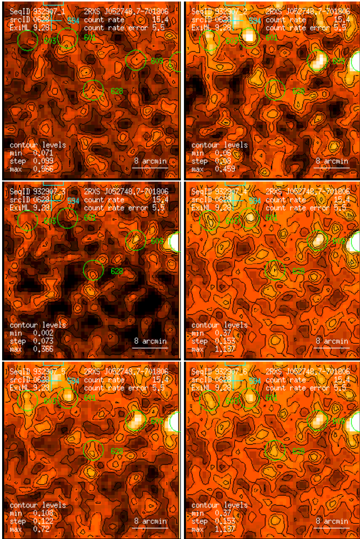
Figure 628: RASS 932907: detection 0628: band rate images, Gaussian filter: (1) PSPC channels 11 – 41, (2) 52 – 90, (3) 91 – 201, (4) 11 – 235, (5) 52 – 201, (6) 11 – 201. Broad band rates in counts/ks. Band rate contour levels in counts/ks/arcmin 2 .
