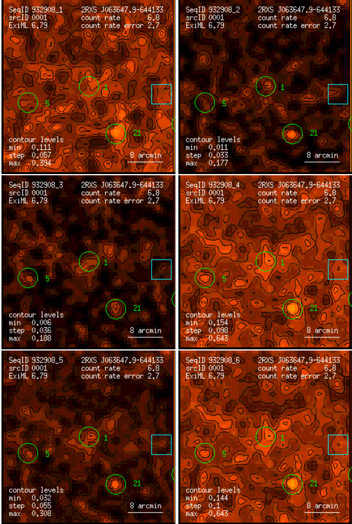
Figure 1: RASS 932908: detection 0001: band rate images, Gaussian filter: (1) PSPC channels 11 – 41, (2) 52 – 90, (3) 91 – 201, (4) 11 – 235, (5) 52 – 201, (6) 11 – 201. Broad band rates in counts/ks. Band rate contour levels in counts/ks/arcmin 2 .
