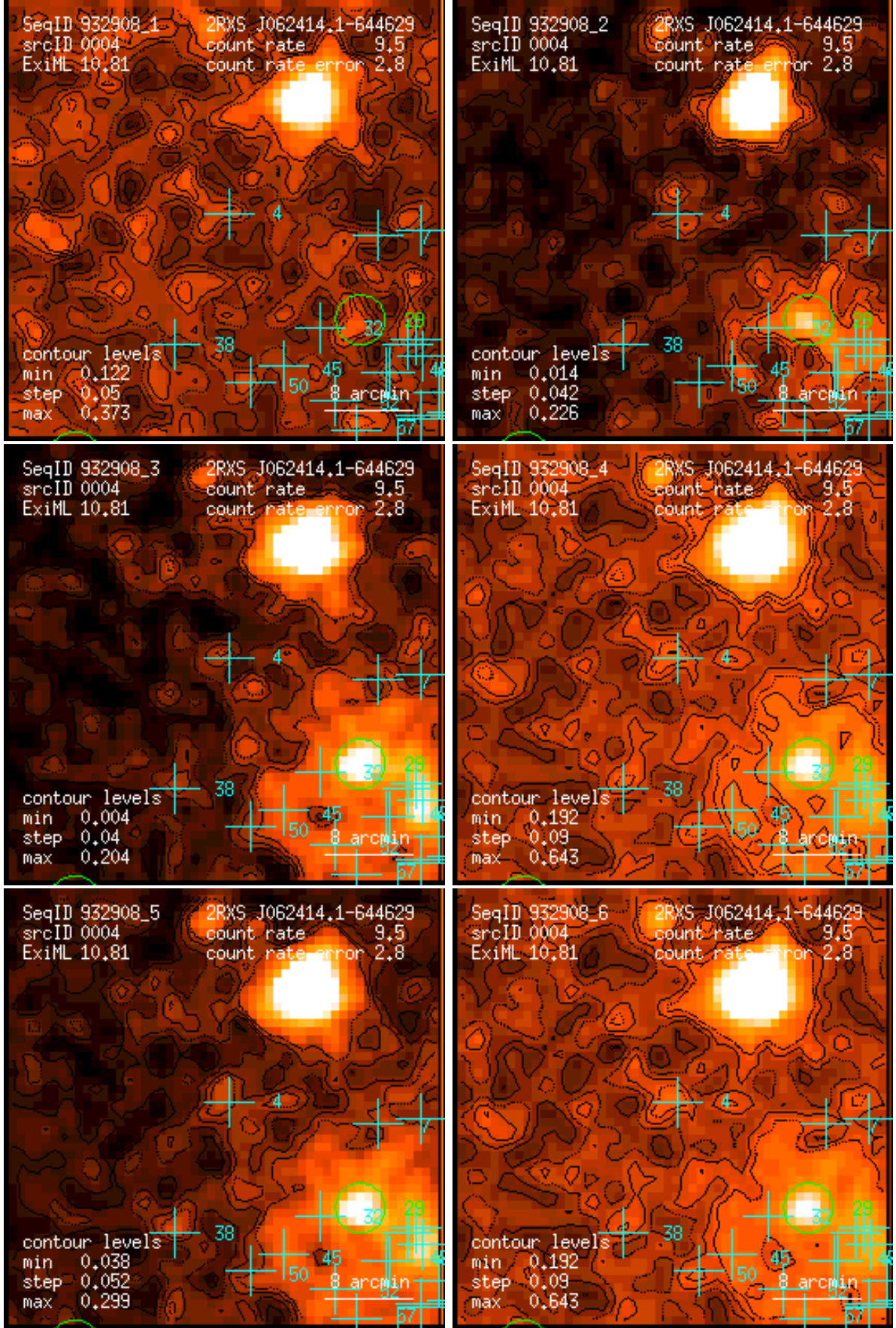
Figure 4: RASS 932908: detection 0004: band rate images, Gaussian filter: (1) PSPC channels 11 – 41, (2) 52 – 90, (3) 91 – 201, (4) 11 – 235, (5) 52 – 201, (6) 11 – 201. Broad band rates in counts/ks. Band rate contour levels in counts/ks/arcmin 2 .
