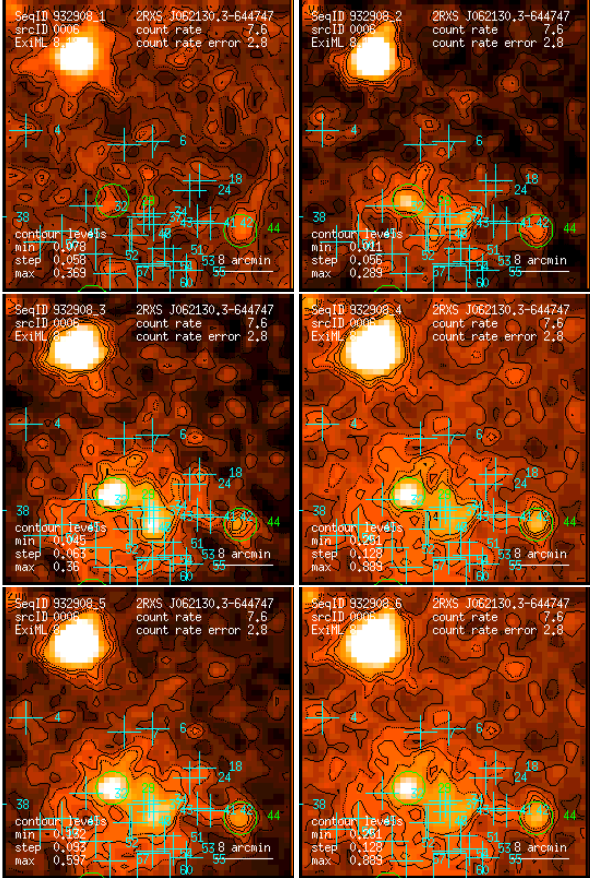
Figure 6: RASS 932908: detection 0006: band rate images, Gaussian filter: (1) PSPC channels 11 – 41, (2) 52 – 90, (3) 91 – 201, (4) 11 – 235, (5) 52 – 201, (6) 11 – 201. Broad band rates in counts/ks. Band rate contour levels in counts/ks/arcmin 2 .
