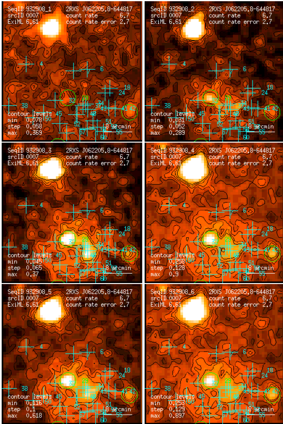
Figure 7: RASS 932908: detection 0007: band rate images, Gaussian filter: (1) PSPC channels 11 – 41, (2) 52 – 90, (3) 91 – 201, (4) 11 – 235, (5) 52 – 201, (6) 11 – 201. Broad band rates in counts/ks. Band rate contour levels in counts/ks/arcmin 2 .
